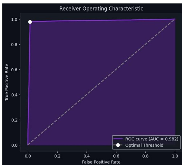
Fig. 3. ROC curve of the proposed Stacking Ensemble.
