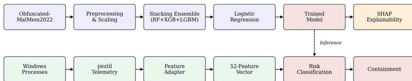
Fig. 1. Architecture of the proposed memory-based malware detection framework with SHAP explainability, Windows live monitoring, feature adaptation, and containment.
