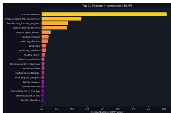
Fig. 4. Global SHAP feature importance of the proposed malware detection model.
