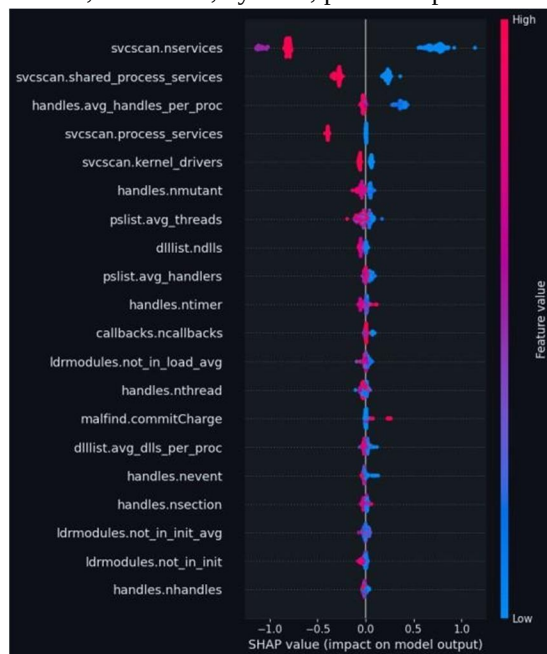
Fig. 5. SHAP waterfall explanation for a representative prediction.
