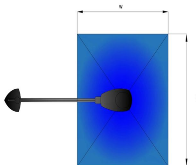
Fig.8 (a) (b) (c) Street Light geometrical parameters.
