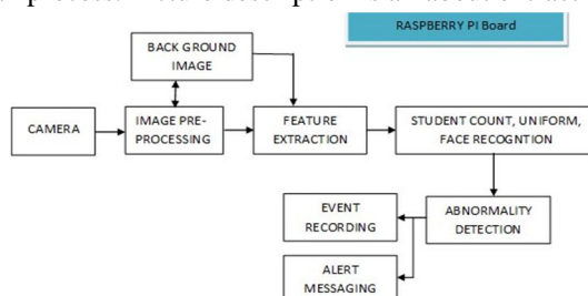
Fig.2.Procedures of Face Detection
