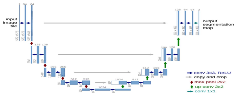
Fig. 2.4. U-Net architecture
