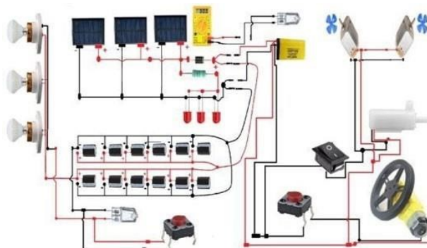
Fig. 2. Connection diagram
