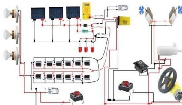
Fig. 2. Connection diagram
