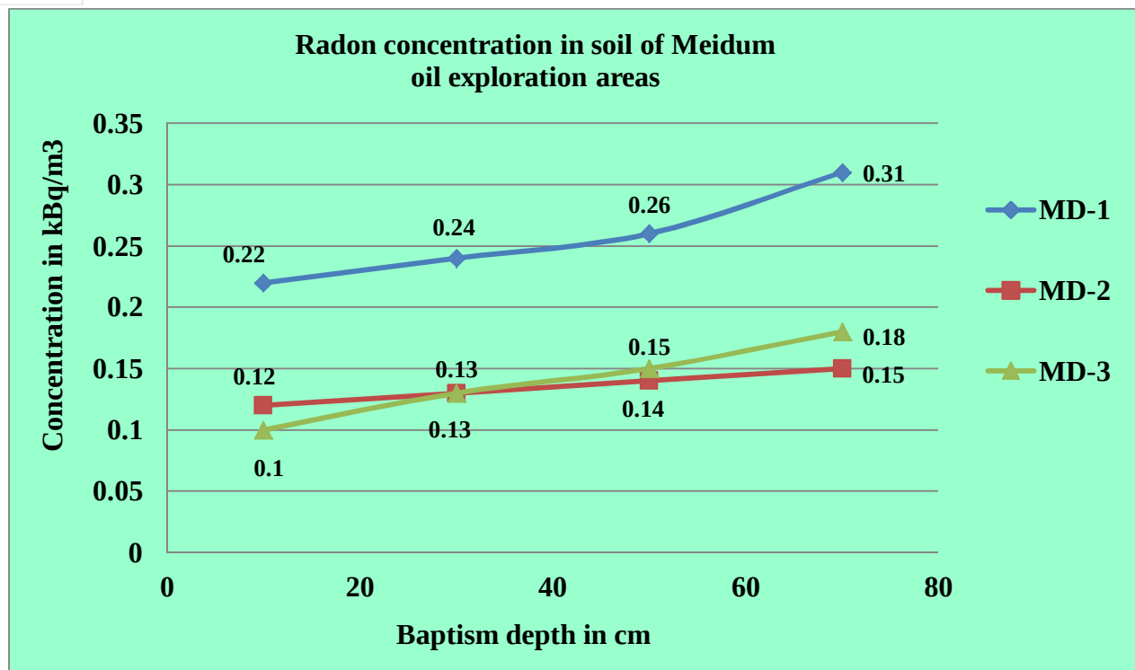
Graph-1. Radon concentration at different depth in soil of Meidum oil exploration area
