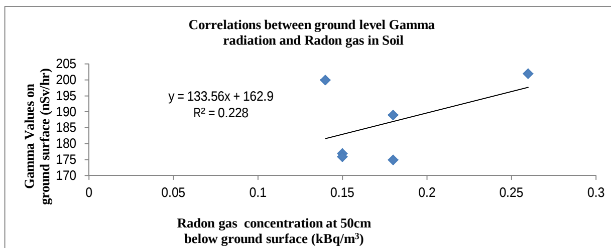
Graph-5. Correlation between Ground level gamma radiation and Radon concentration at 50cm deep.
