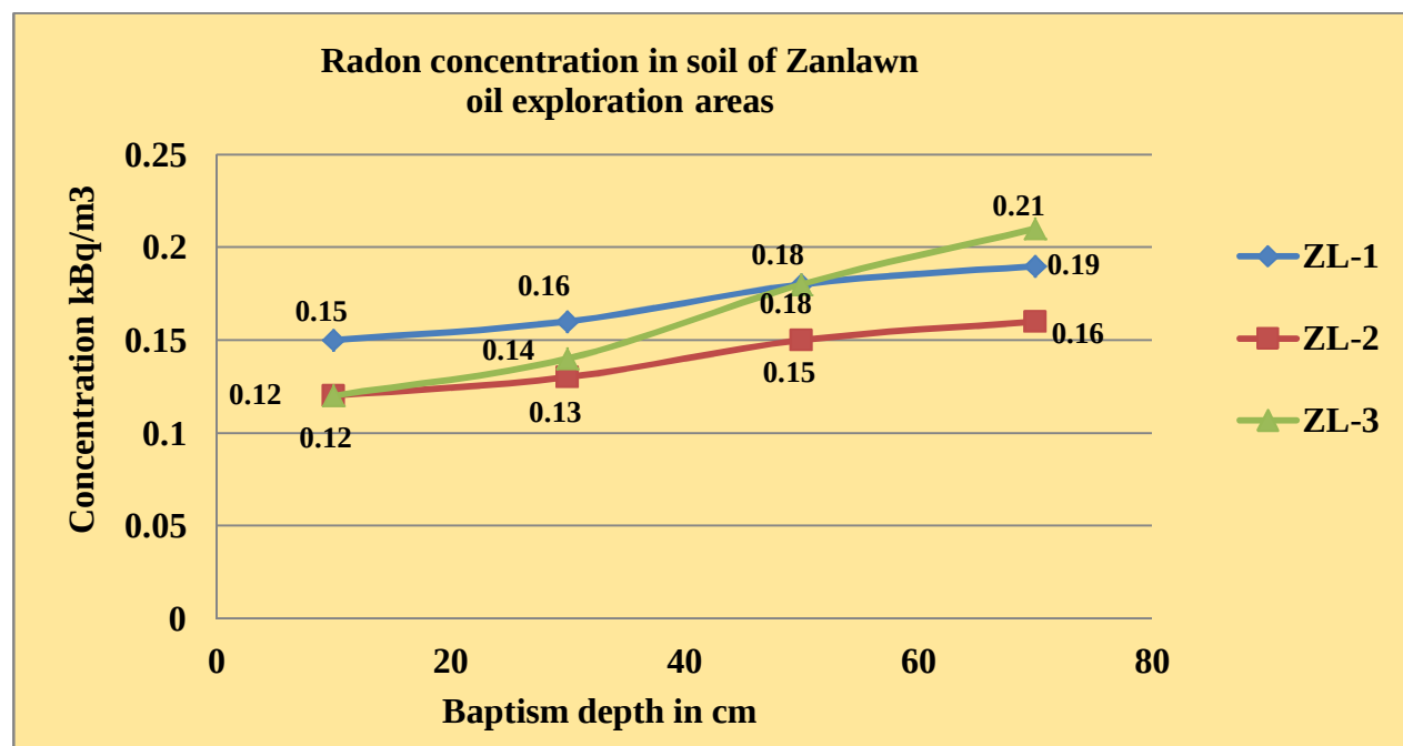
Graph-2. Radon concentration at different depth in soil of Zanlawn oil exploration area
