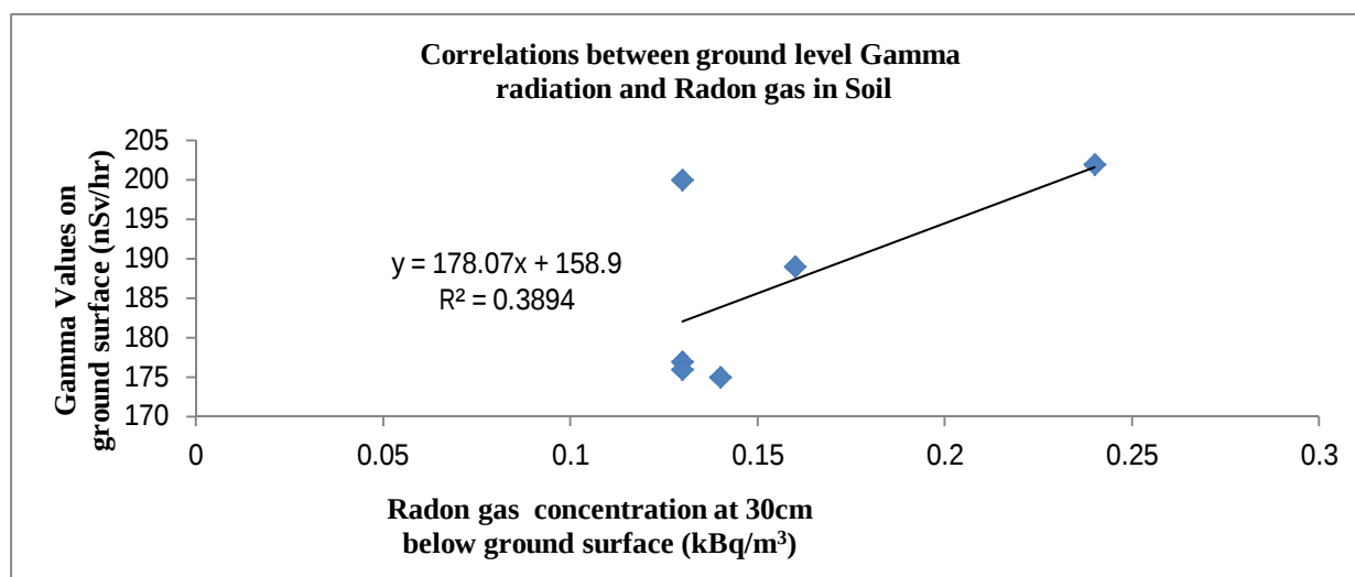
Graph-4. Correlation between Ground level gamma radiation and Radon concentration at 30cm deep.
