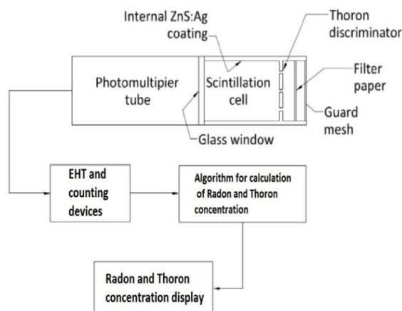
Fig.4. Block diagram of Smart RnDuo
