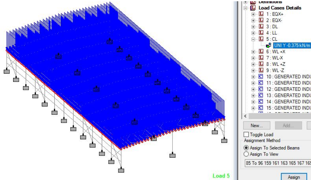
Figure 15: Collateral Load
