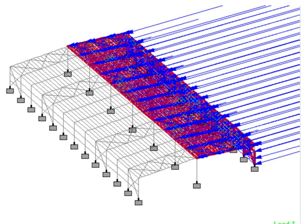
Figure 17: Wind Load (-X Direction)
