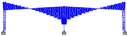
Figure 23: SFD in 25m Span
