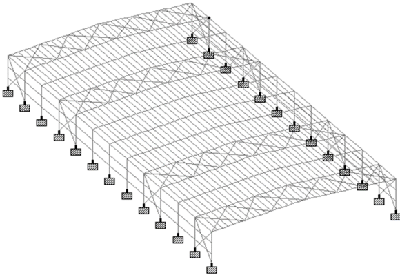
Figure 6: STAAD.Pro model Geometry "A"
