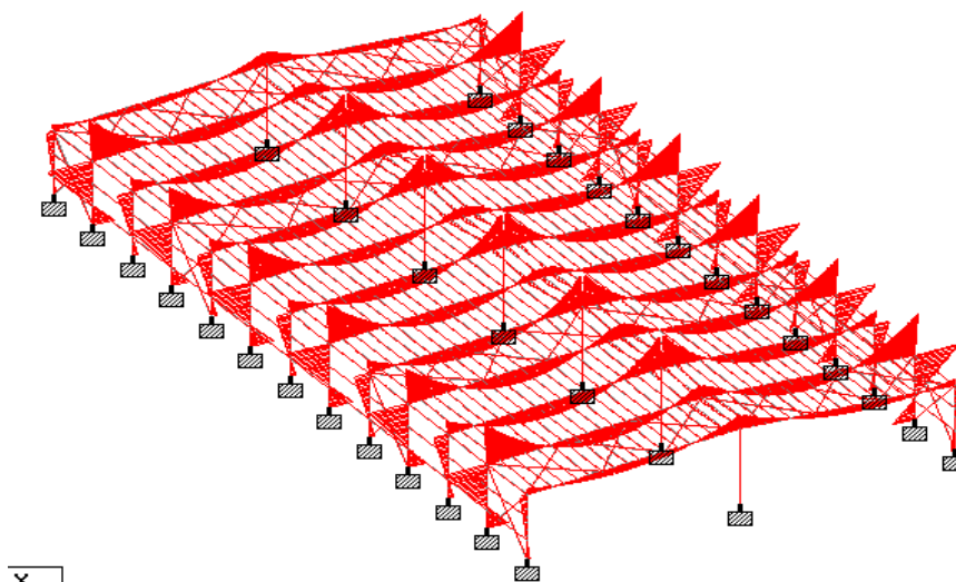
Figure 22: Bending Moment Diagram of whole section
