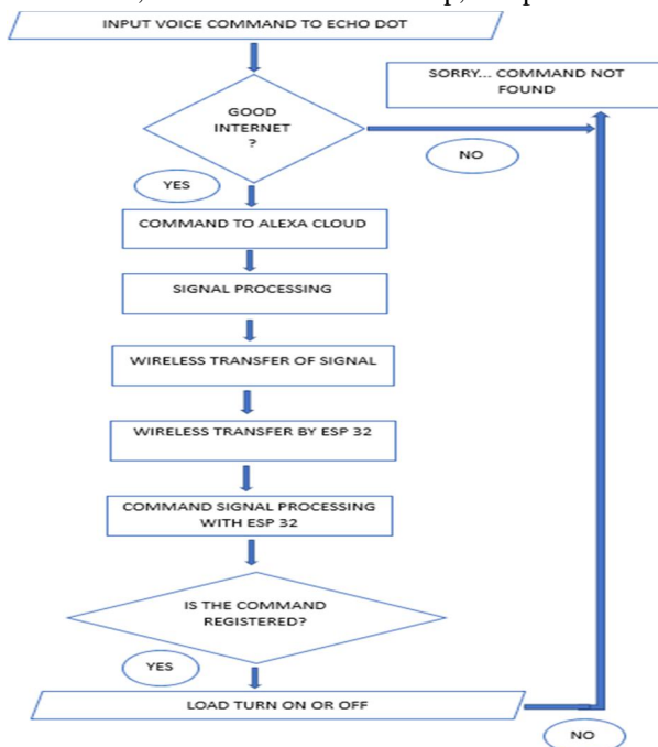
Fig.2 System Flowchart
