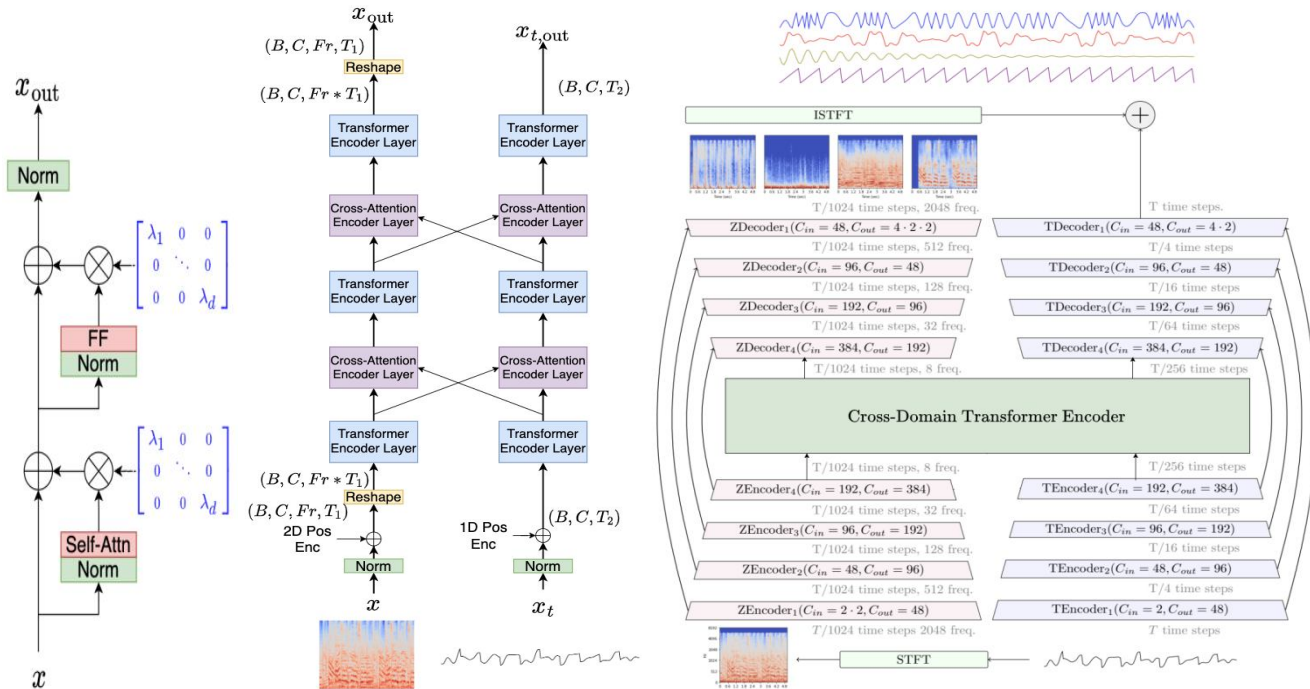
Fig. 1: Details of the Hybrid Transformer Demucs architecture. (a): the Transformer Encoder layer with self-attention and Layer Scale [6]. (b): The Cross-domain Transformer Encoder treats spectral and temporal signals with interleaved Transformer Encoder layers and cross-attention Encoder layers. (c): Hybrid Transformer Demucs keeps the outermost 4 encoder and decoder layers of Hybrid Demucs with the addition of a cross-domain Transformer Encoder between them.
