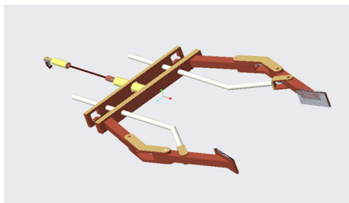
Figure 2 3D angular view of Hydraulic Gripper
