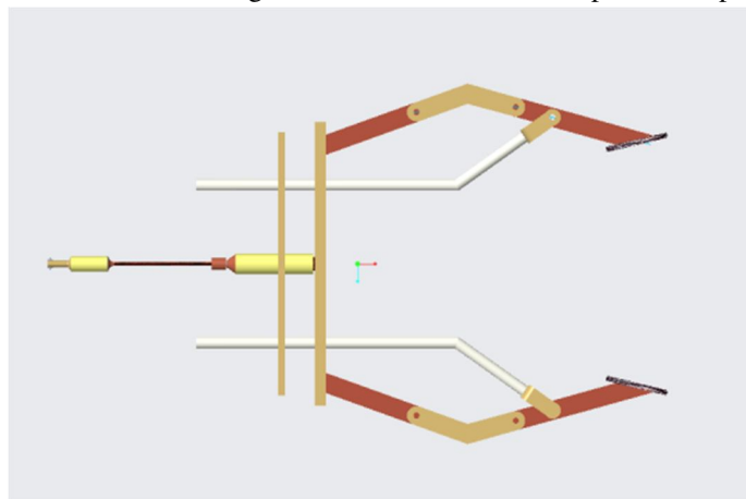
Figure 1 3D Top view of Hydraulic Gripper
