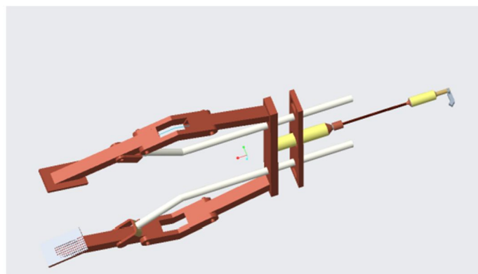
Figure 3 3D angular view of Hydraulic Gripper
