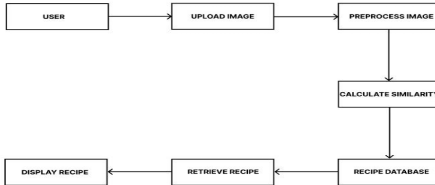
Fig. 1 Methodology
