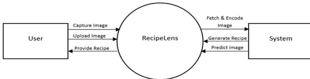
Fig.2 Level 0 DFD
