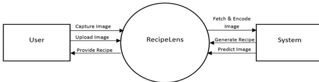
Fig.2 Level 0 DFD
