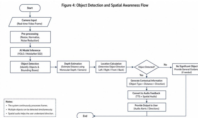
Figure 4: Object Detection Flow
