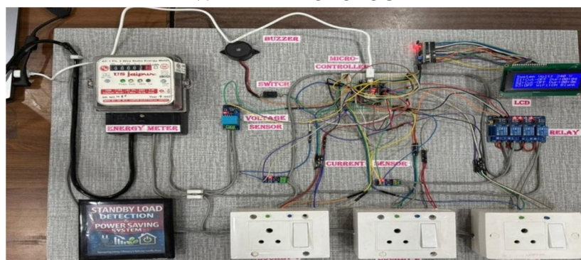
Fig. 2. Hardware Prototype
