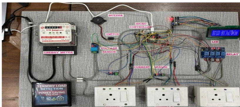
Fig. 2. Hardware Prototype
