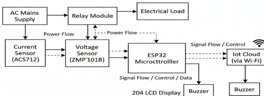
Fig. 1. Block Diagram
