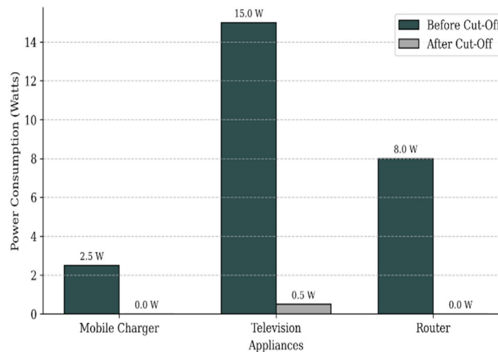
Fig 4. Comparison of Standby Power Consumption Before and After Power Cut-Off
