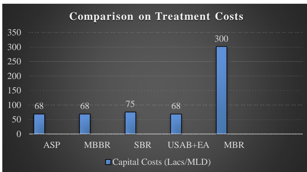
Graph 4.2: Comparison on Treatment Costs
