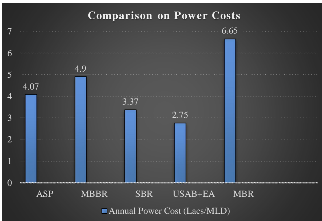
Graph 4.4: Comparison on Power Costs
