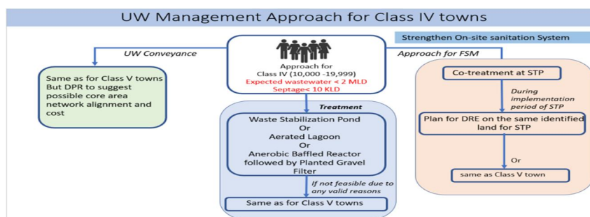
Fig.3.4: UW Management Approach for Class IV towns
