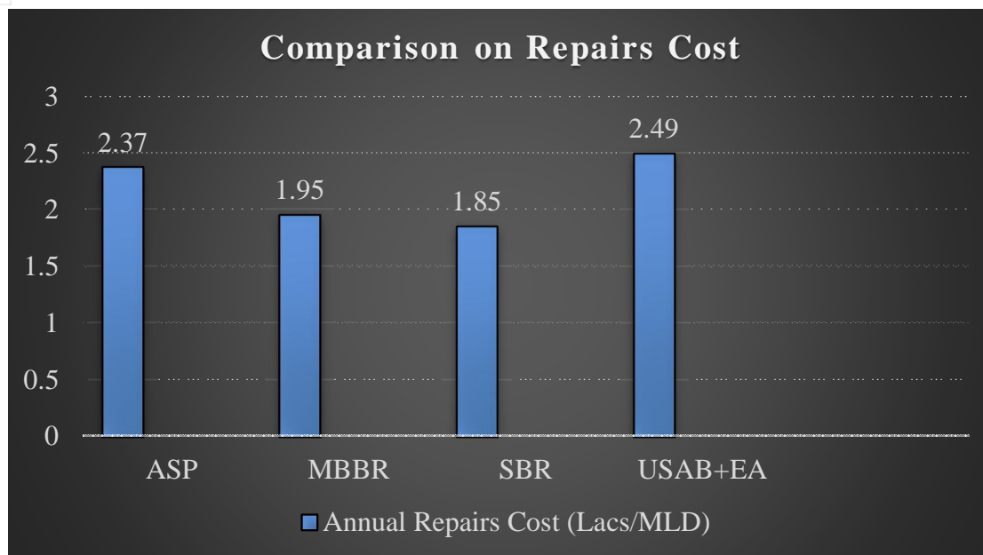
Graph 4.5: Comparison on Repairs Cost
