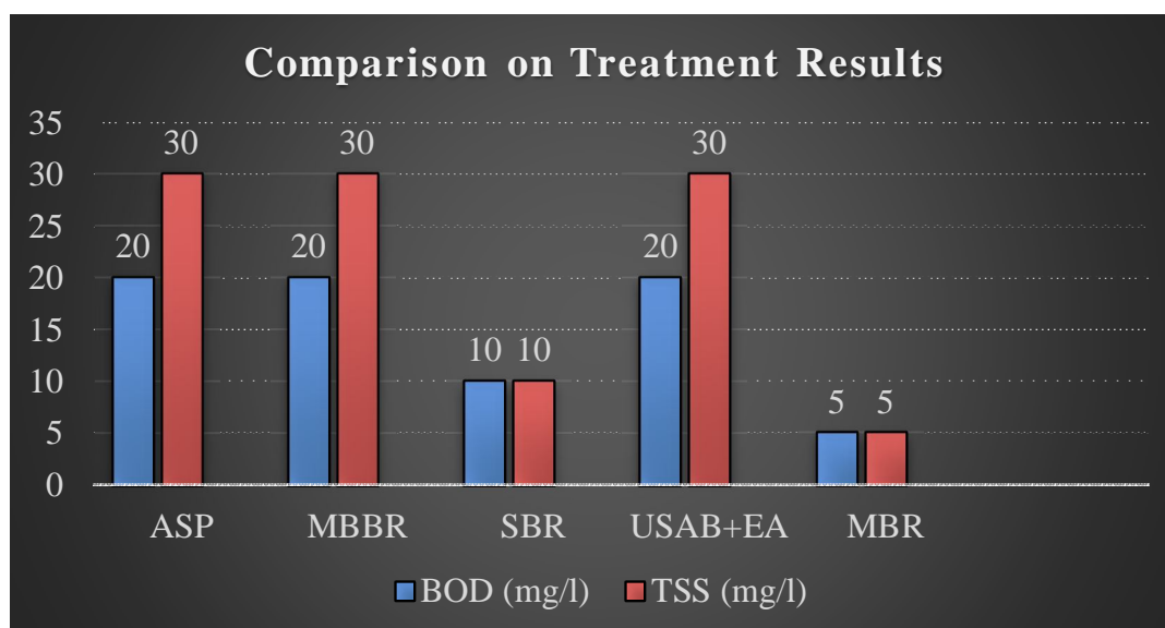
Graph 4.1: Comparison on Treatment Results
