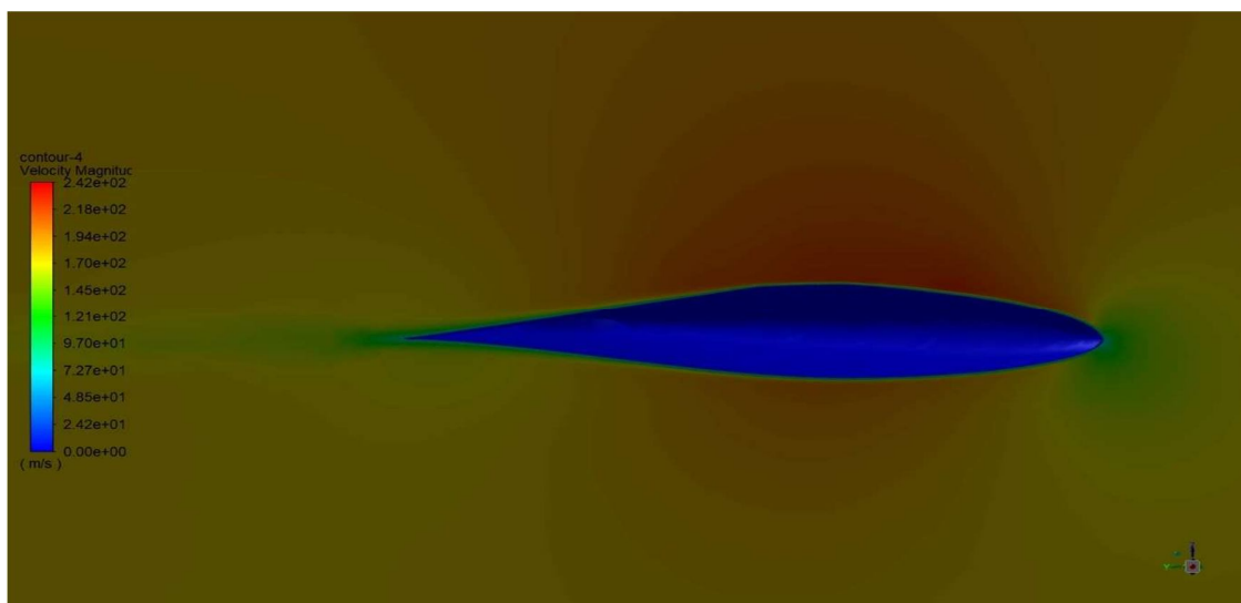
Figure 28 Velocity contour for 10 degree AOA of modified airfoil
