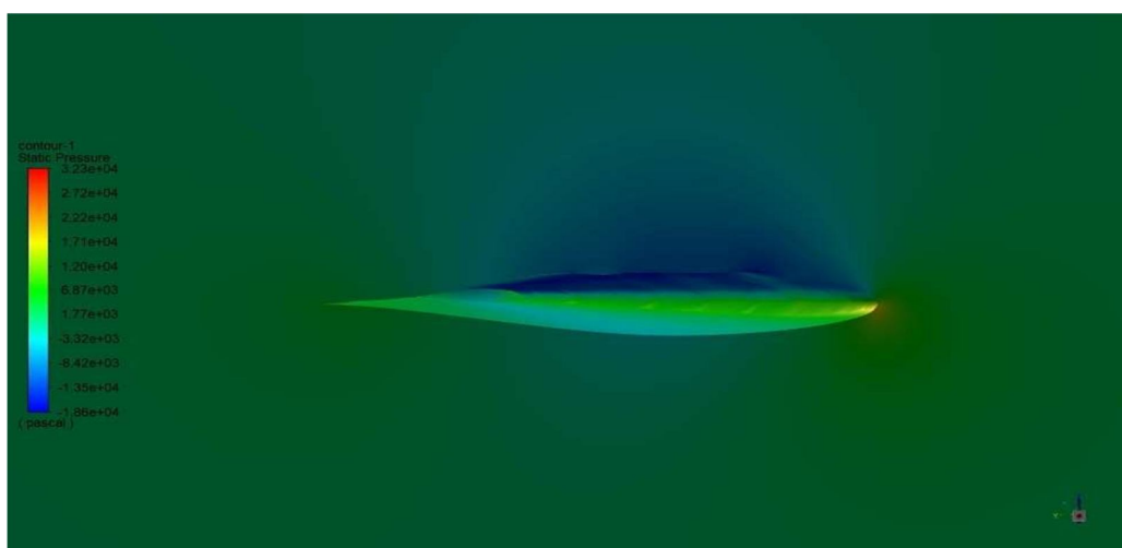
Figure 29 Pressure contour for 15 degree AOA of modified airfoil
