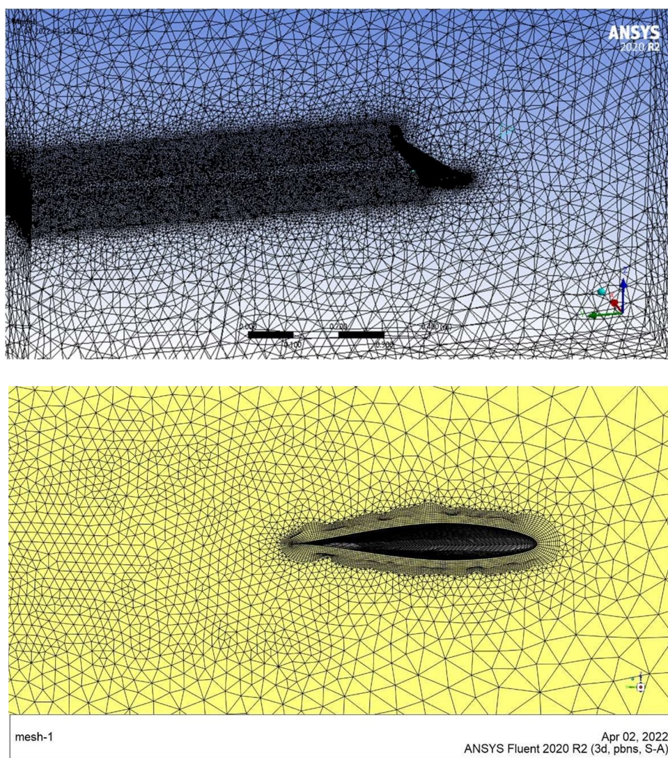
Figure 12 mesh
