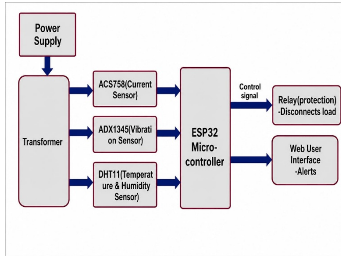
Fig. 1. Figure 1: Block Diagram of Industrial IoT Based Health Monitoring System of Transformer.
