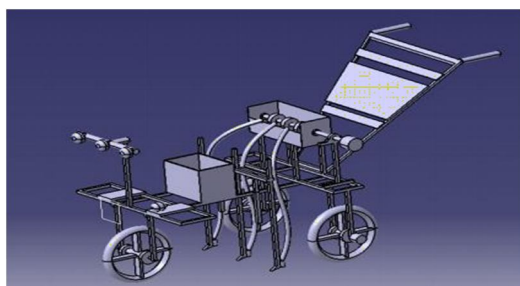
Fig.1: Catia Model
