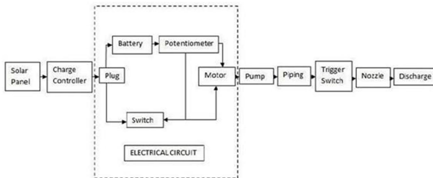
Fig.2: Block diagram of the spraying system
