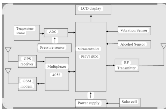
Fig.5.1 Architecture of Smart Helmet for Accident and Safety Alert
