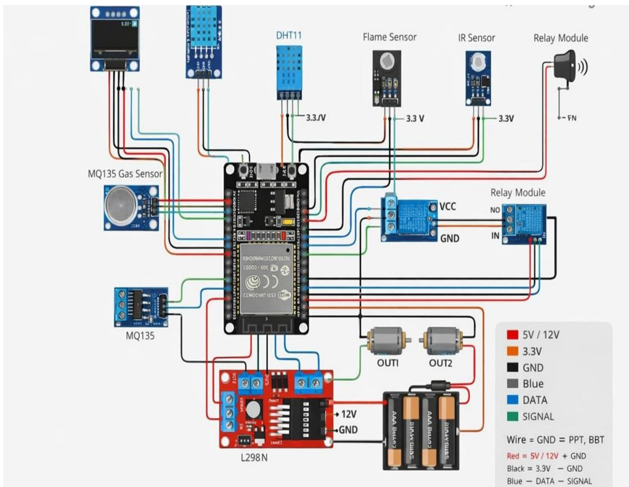
Fig.1 Circuit Diagram
