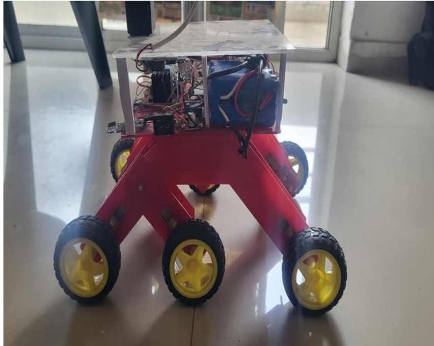
Fig. 2 System Photo
