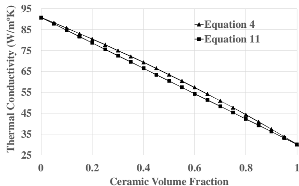
Figure 1. Thermal conductivity of nickel-alumina material using the model from Equation 4 and that from a proportional law of mixtures, given in Equation 11
