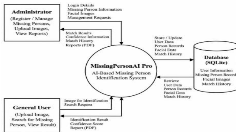
Figure 2: Context Diagram of MissingPersonAI Pro
