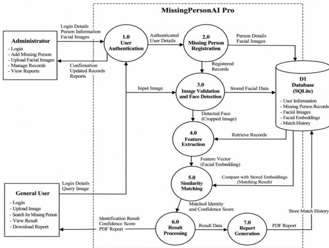
Fig. 4: Data Flow Diagram (DFD) of MissingPersonAI Pro
