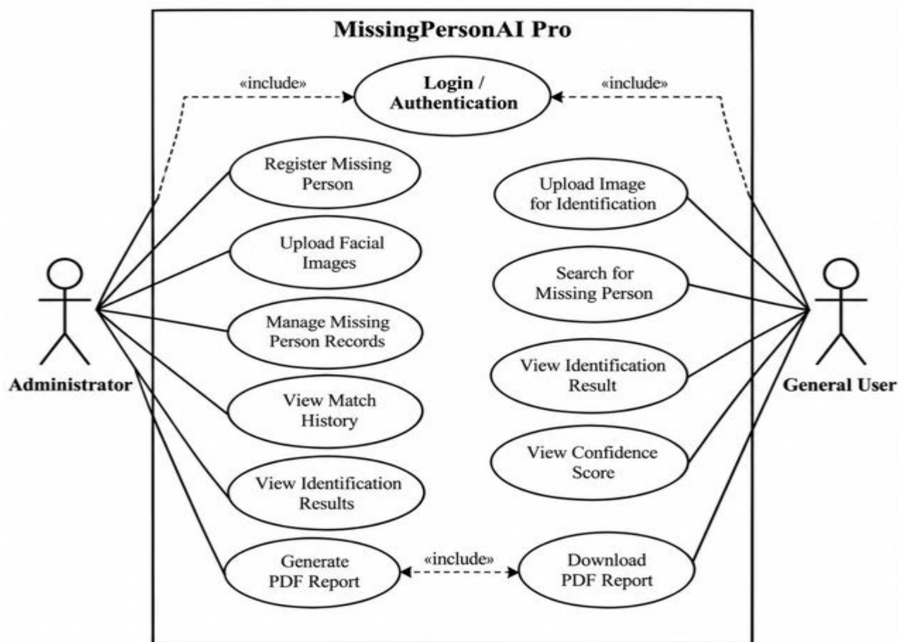
Fig. 3: Use Case Diagram of MissingPersonAI Pro
