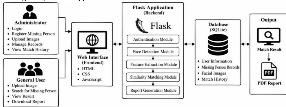
Figure 1: System Architecture of MissingPersonAI Pro
