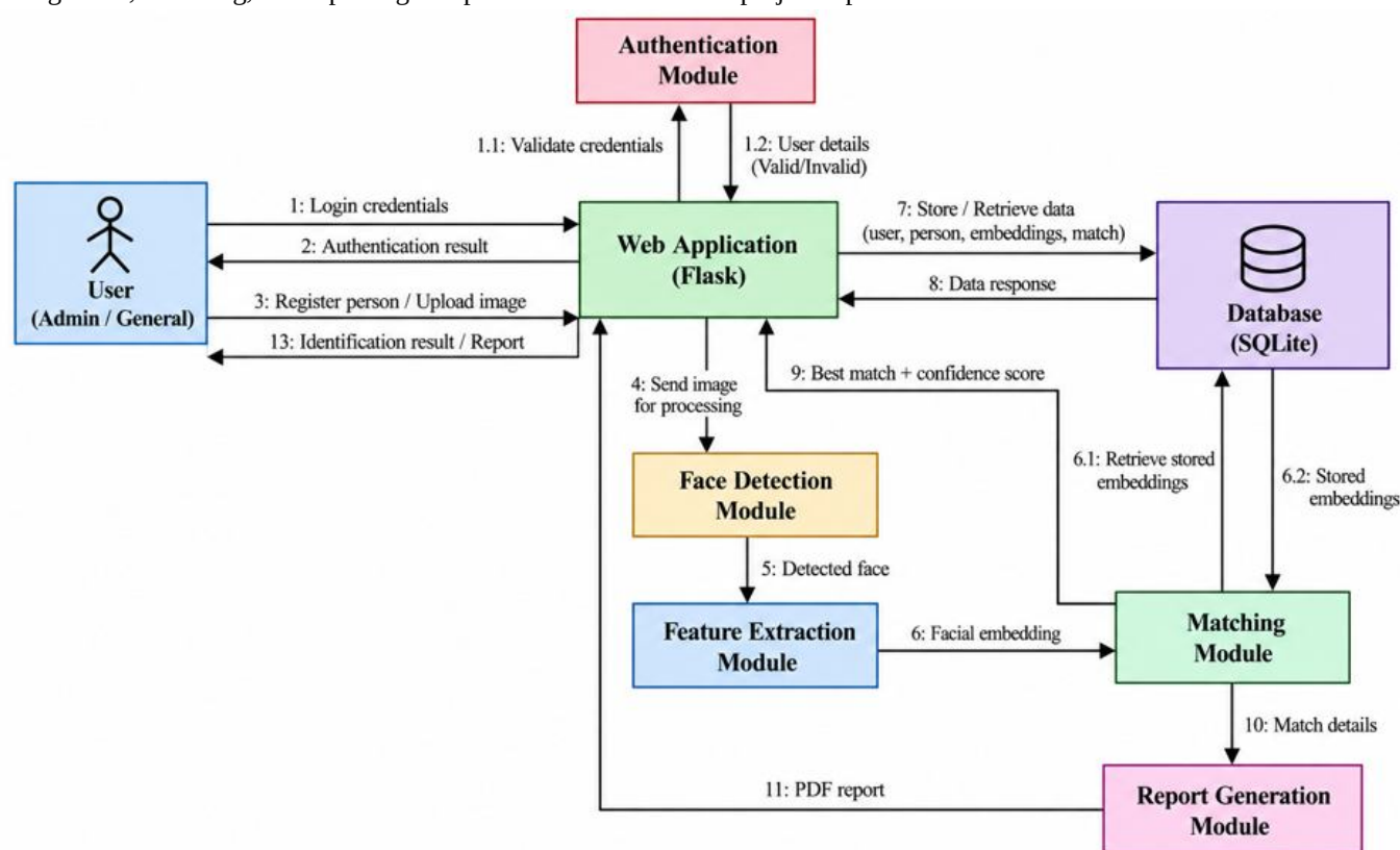
Fig. 6 Collaboration Diagram
