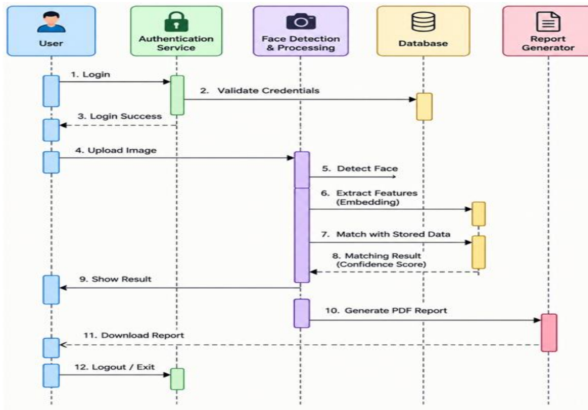
Fig.5 Sequence Diagram
