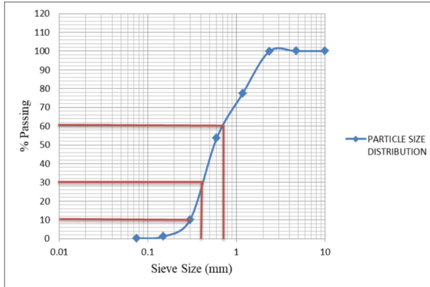
Fig. 1 Sieve analysis of sand
