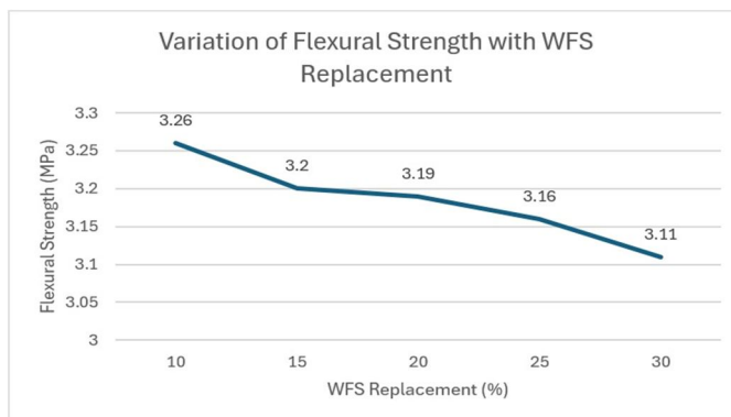
Figure 4 : Graph of Flexural Strength V/S WFS Replacement
