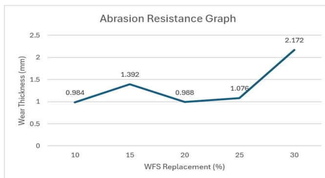
Figure 5 : Graph of Wear Thickness V/S WFS Replacement
