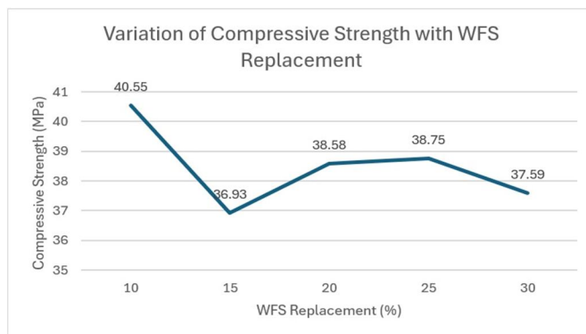
Figure 2 : Graph of Compressive Strength V/S WFS Replacement
