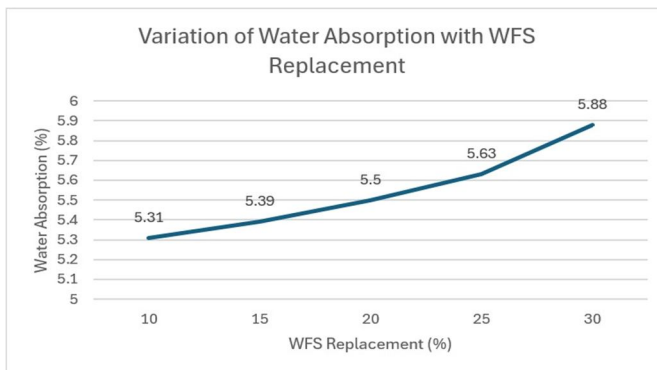
Figure 3 : Graph of Water Absorption V/S WFS Replacement
