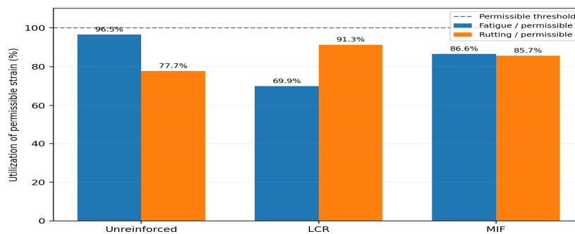
Figure 12. Percentage utilization of the permissible fatigue and rutting strain limits.
