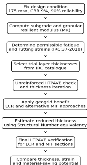
Figure 1. Research methodology adopted for the unreinforced, LCR-reinforced and MIF-reinforced pavement analyses.
