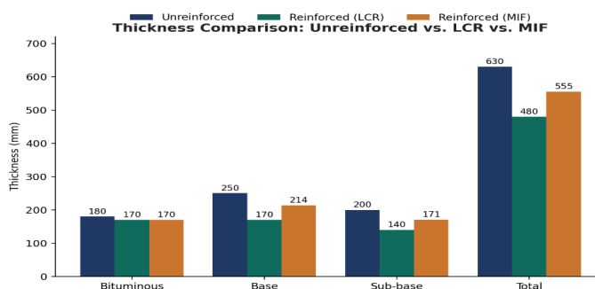
Figure 9. Layer and total thickness comparison for unreinforced, LCR and MIF designs.
