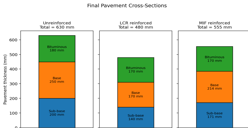
Figure 13. Corrected schematic comparison of the final pavement cross-sections
