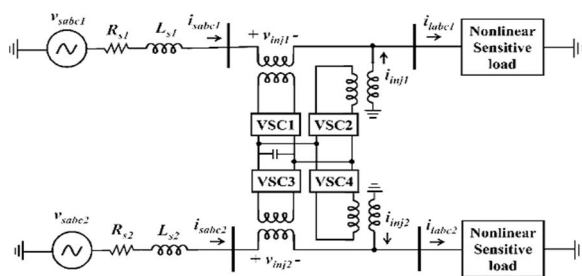
Fig2: Single line diagram Of four converter
