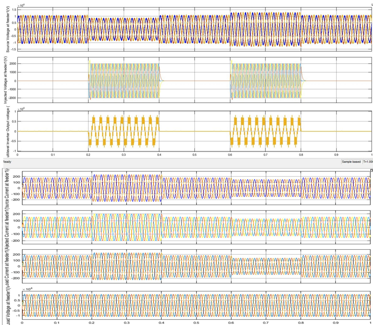
Fig 15: Voltages and currents at feeder 1
