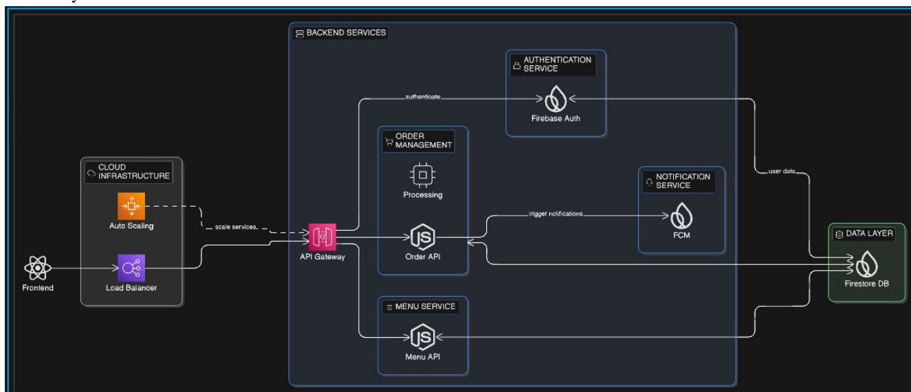
Fig.3 Backend Flowchart
