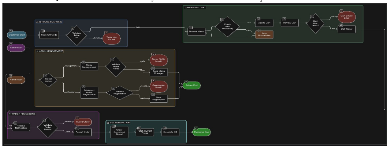
Fig.1Flowchart for QR-based Restaurant menu
