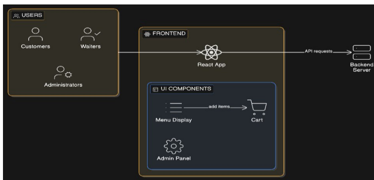
Fig.2 Frontend Flowchart
