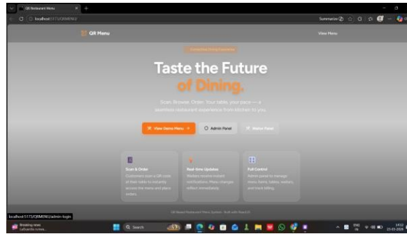
Fig.5 gateway interface
