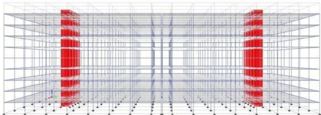
Figure: Elevation View of G+9 Structure of 90m slab length with expansion joint.
