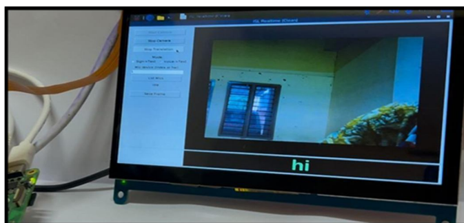
Fig. 2. “Speech-to-Text”
