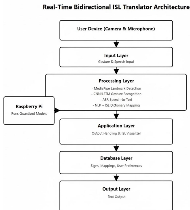
Fig. 1. “System Architecture of Bidirectional Translator”
