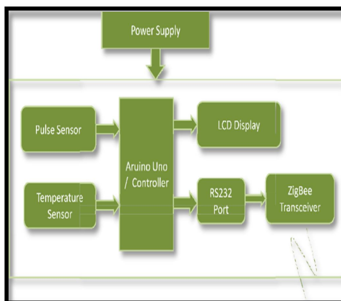
Fig.1 Block Diagram of Transmitter
