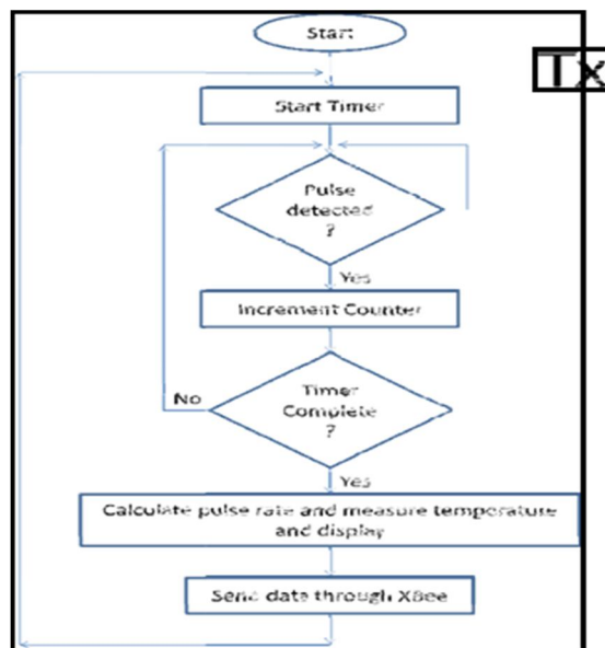
Fig.3 Flow Chart of Transmitter
