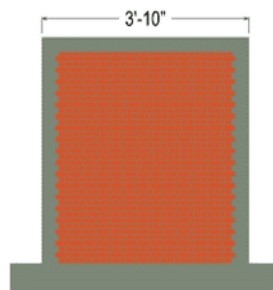
Figure 1. Confined Masonry Single Panel
