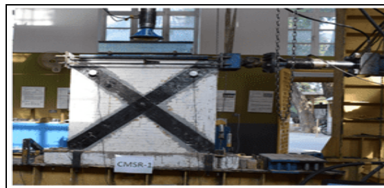
Figure 4. Load setup and instrumentation details
