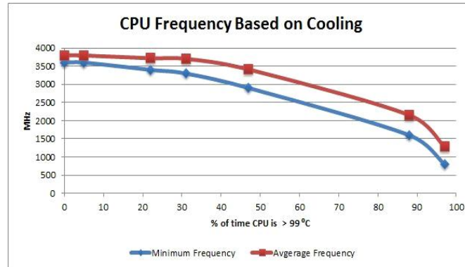
Figure 2. Material vs Cooling Performance
