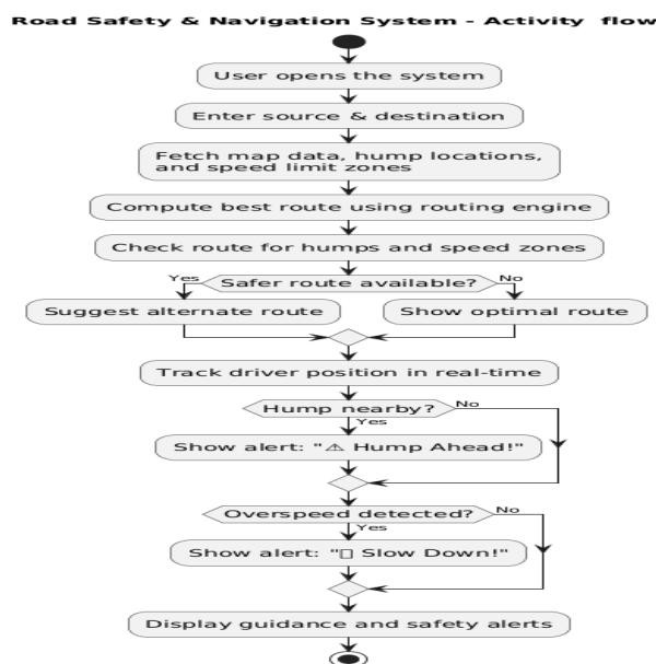
Fig. 1 Activity Diagram of Proposed System
