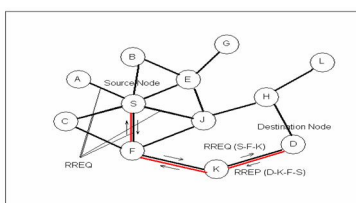
Figure 1 basic principle of Dynamic Source Routing
