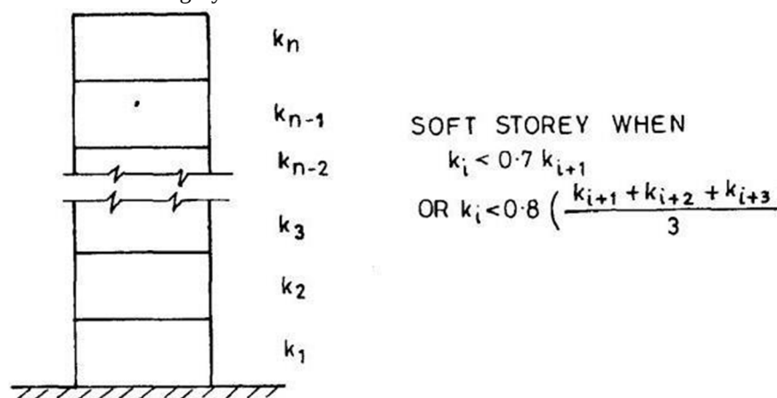
Fig. 1.6 Stiffness Irregularity
