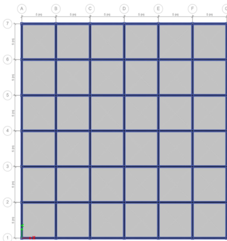
Fig. 3.2 (a) Plan of RF
