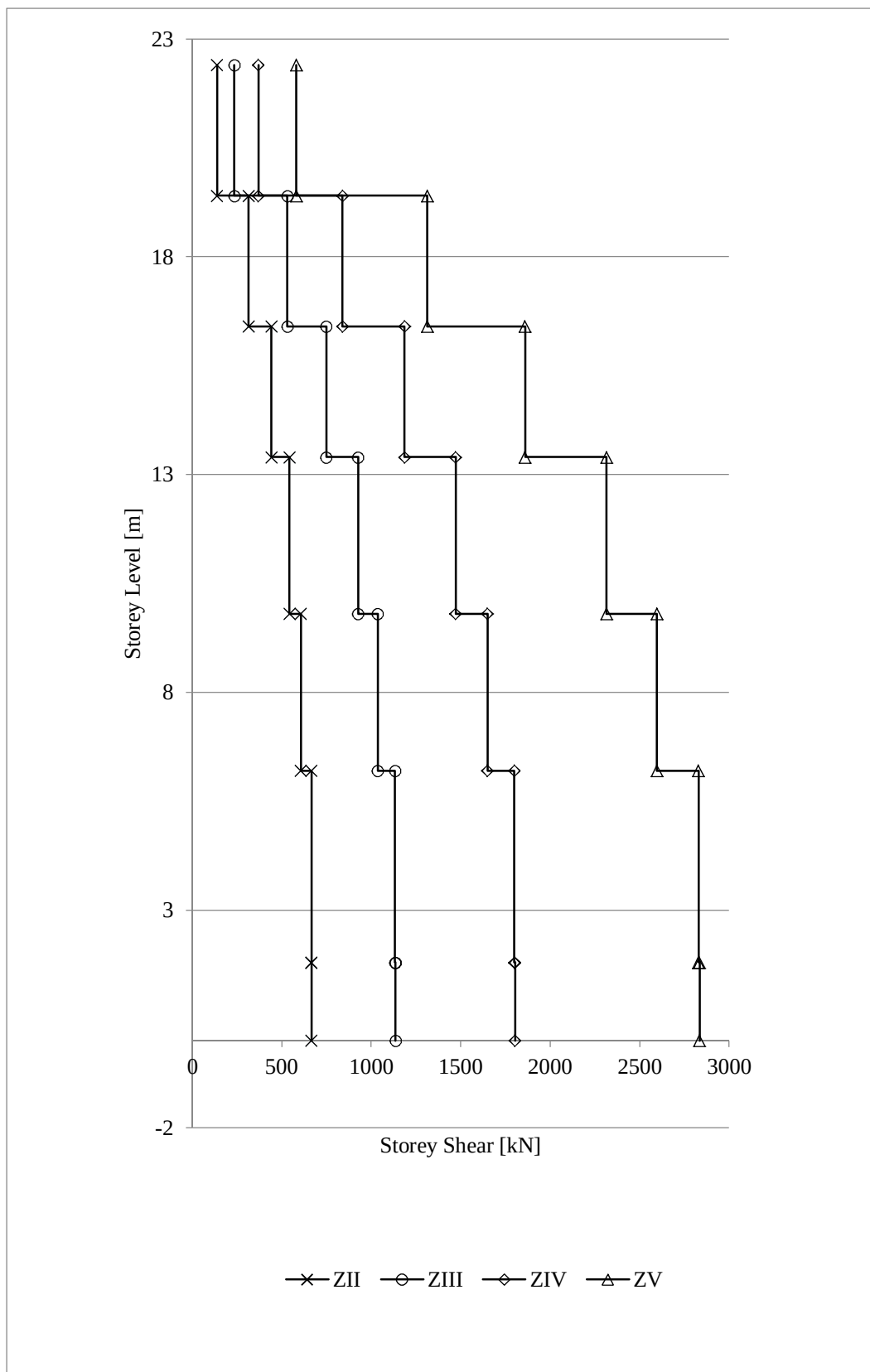
Fig. 4.6 Seismic Response (Storey Shear) of Stiffness Irregular Frame - SIF at all Seismic Zones in India
