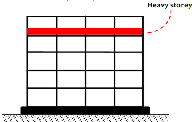
Fig. 1.7 Mass Irregularity
