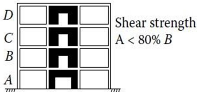
Fig.1.10 Discontinuity in Lateral Strength weak storey Irregularity
