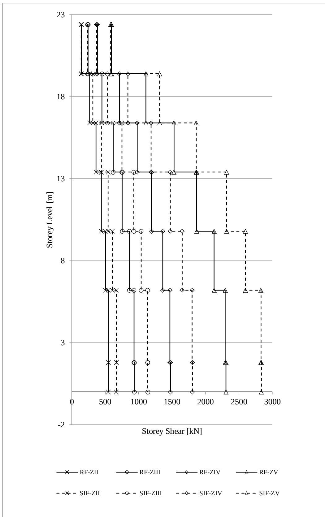
Fig. 4.9 Storey Shear Response of Regular (RF) and Stiffness Irregular (SIF) Frames under Seismic Loads
