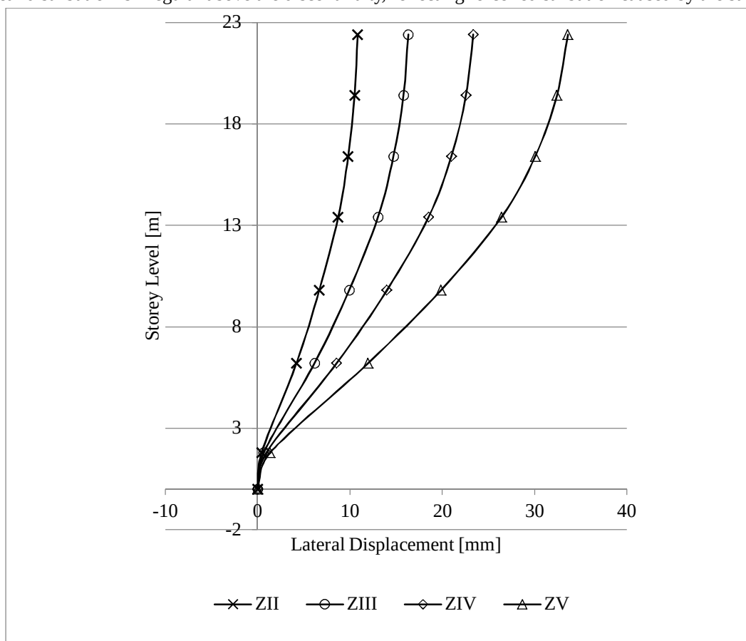
Fig. 4.4 Seismic Response (Lateral Displacement) of Stiffness Irregular Frame - SIF at all Seismic Zones in India
