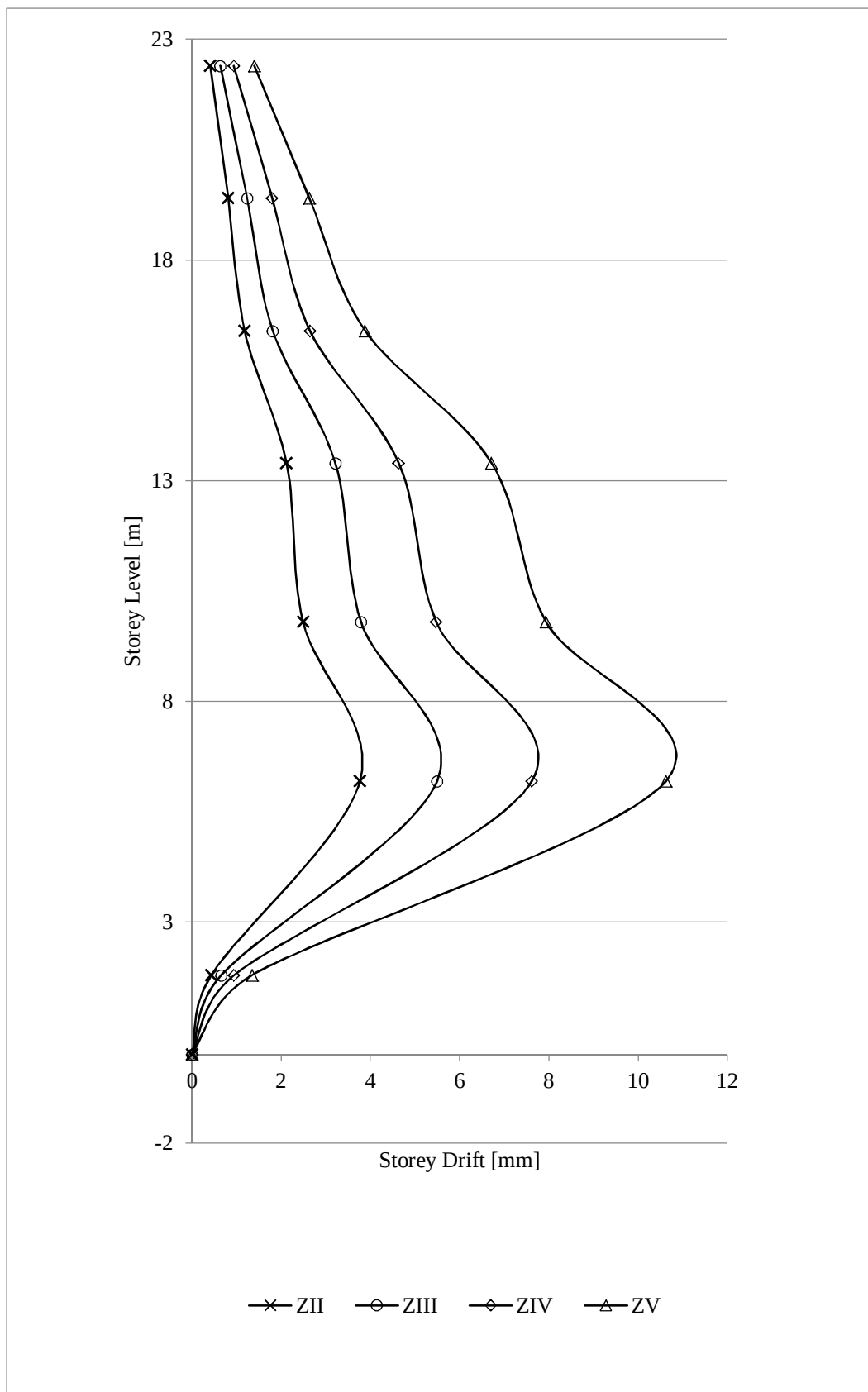
Fig. 4.5 Seismic Response (Storey Drift) of Stiffness Irregular Frame - SIF at all Seismic Zones in India
