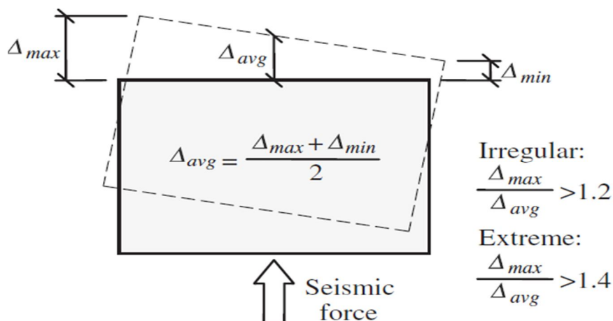
Fig. 1.1 Torsional irregularity
