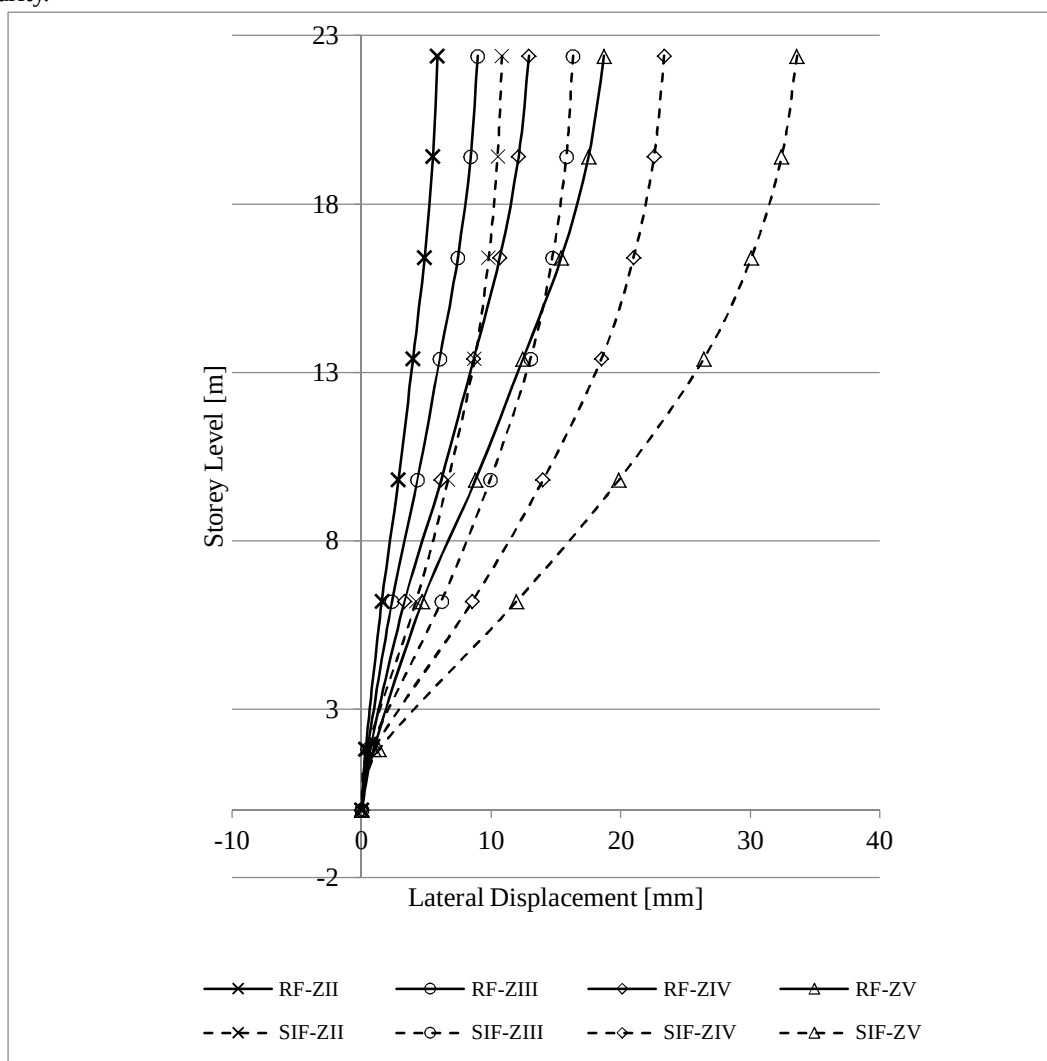
Fig. 4.7 Lateral Displacement Response of Regular (RF) and Stiffness Irregular (SIF) Frames under Seismic Loads
