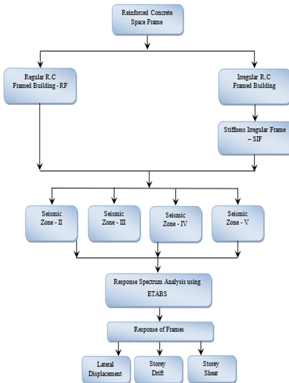
Fig. 3.1 Methodology Flow Chart
