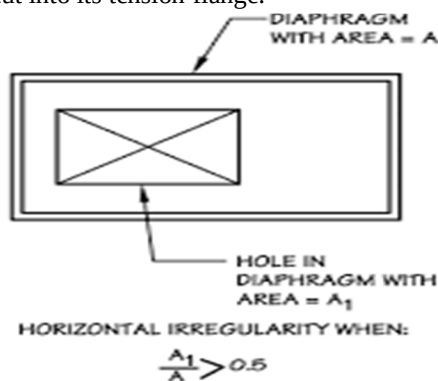
Fig. 1.3 Diaphragm Discontinuity
