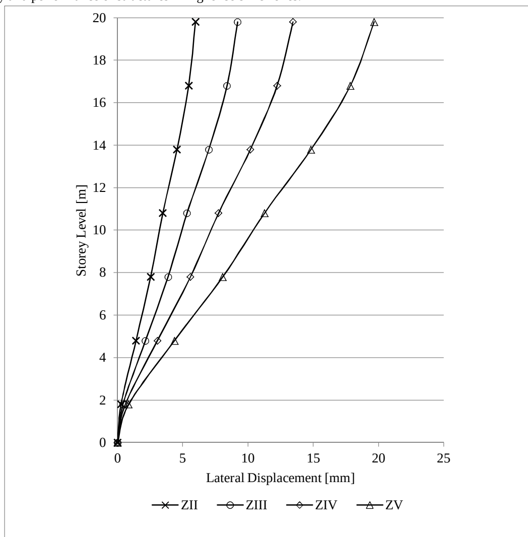
Fig. 4.1 Seismic Response (Lateral Displacement) of Regular Frame – RF at all Seismic Zones in India
