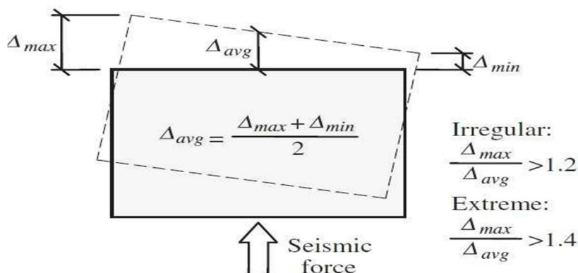
Fig. 1.1 Torsional irregularity
