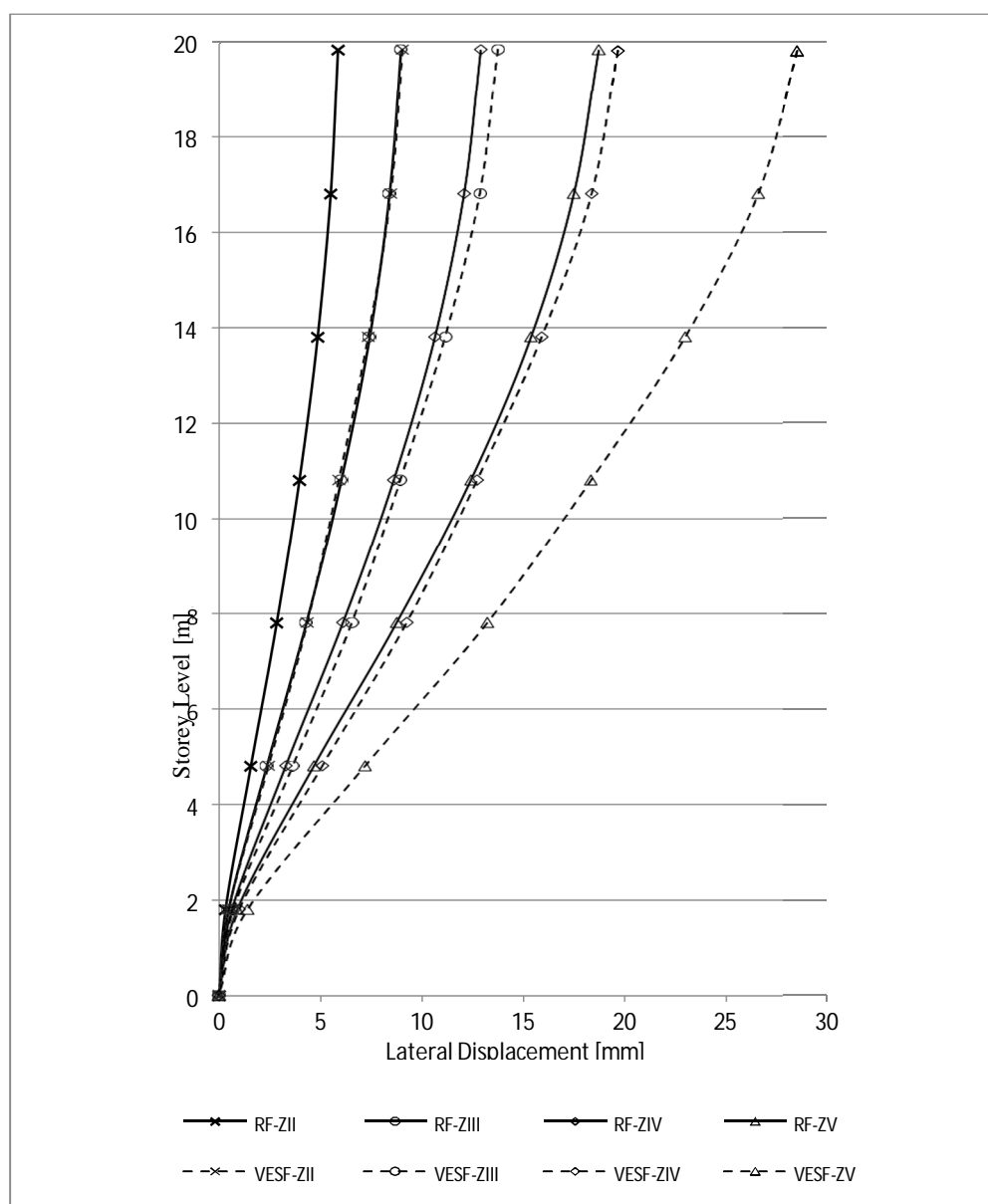
Fig. 4.7 Lateral Displacement Response of Regular (RF) and Vertical Equal & Single Setback (VESF) Frames under Seismic Loads
