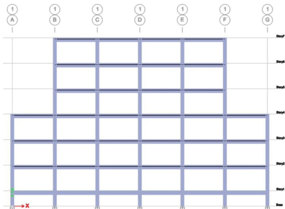
Fig. 3.3 (b) Elevation of VESF
