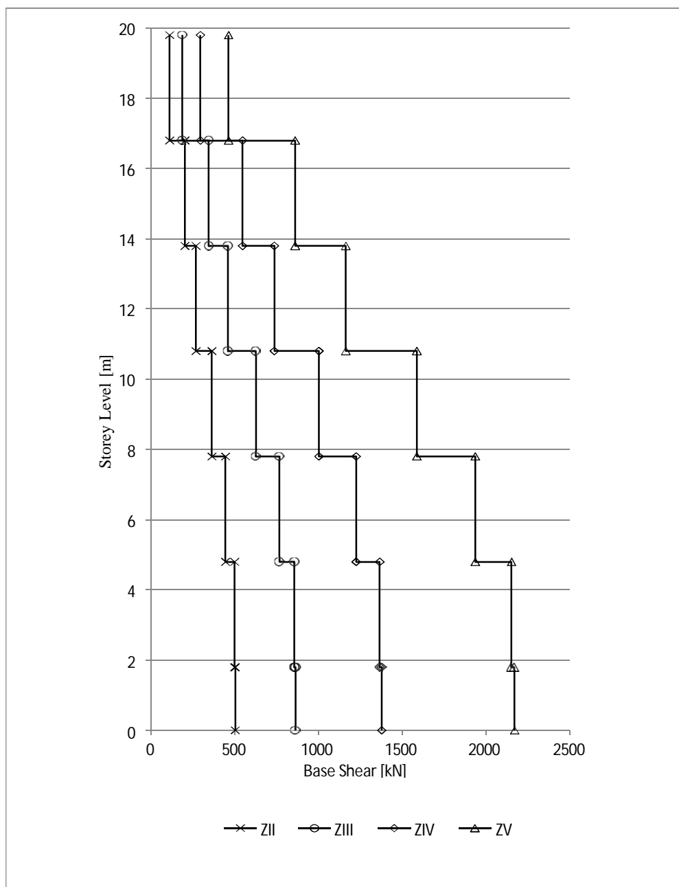
Fig. 4.3 Seismic Response (Storey Shear) of Regular Frame – RF at all Seismic Zones in India
