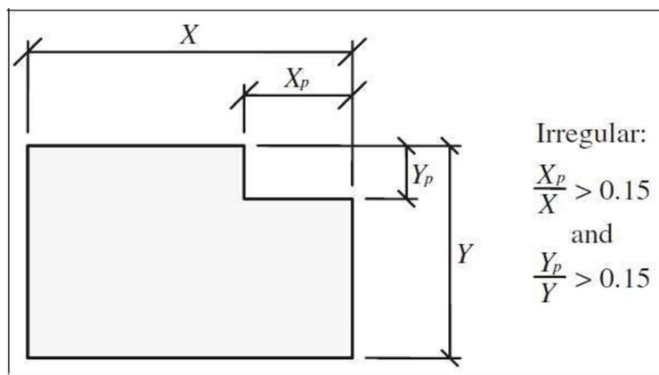
Fig. 1.2 Re-entrant irregularity
