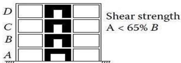
Fig. 1.11 Discontinuity in Lateral Strength Extreme weak storey Irregularity
