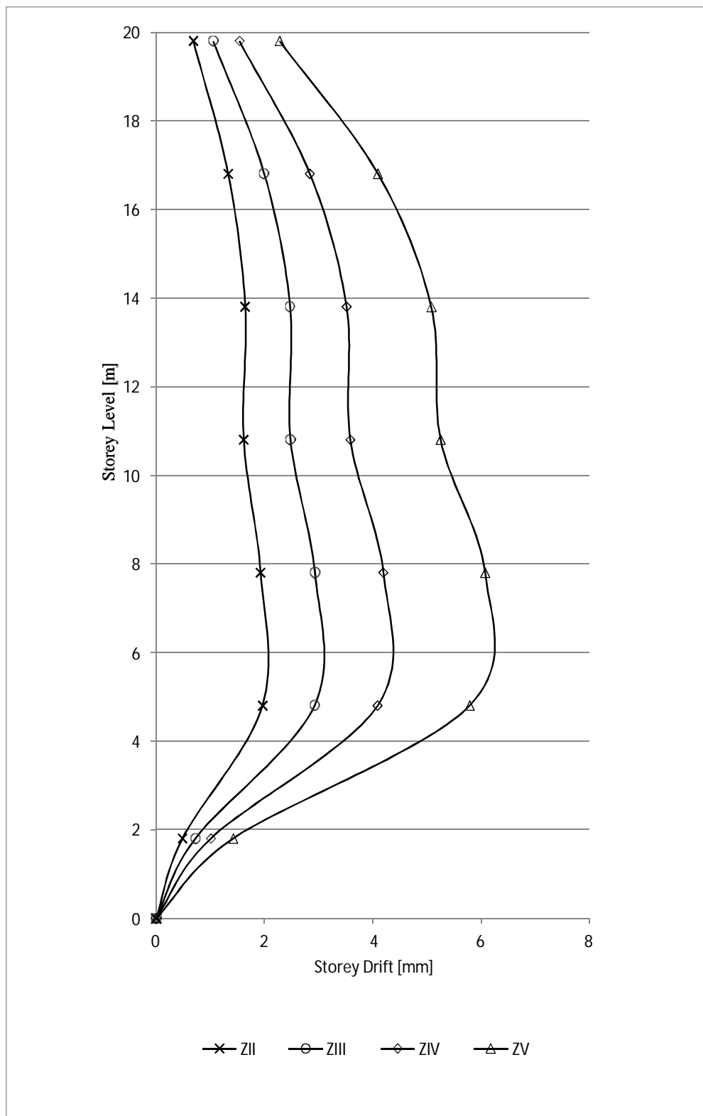
Fig. 4.5 Seismic Response (Storey Drift) of Vertical Equal & Single Setback Frame – VESF at all Seismic Zones in India
