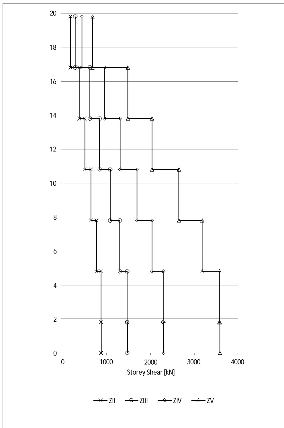
Fig. 4.6 Seismic Response (Storey Shear) of Vertical Equal & Single Setback Frame – VESF at all Seismic Zones in India
