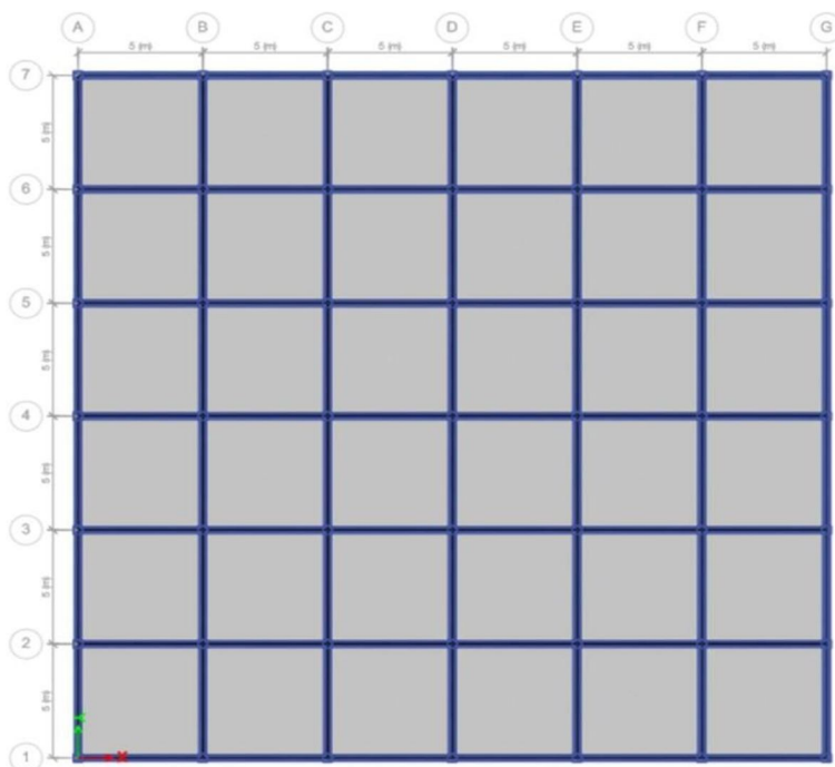
Fig. 3.2 (a) Plan of RF
