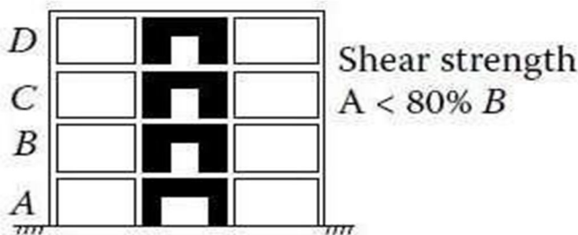
Fig.1.10 Discontinuity in Lateral Strength weak storey Irregularity
