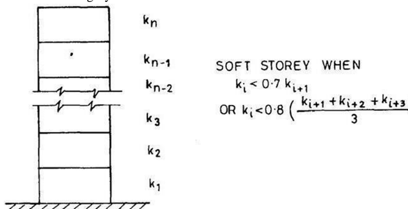
Fig. 1.6 Stiffness Irregularity
