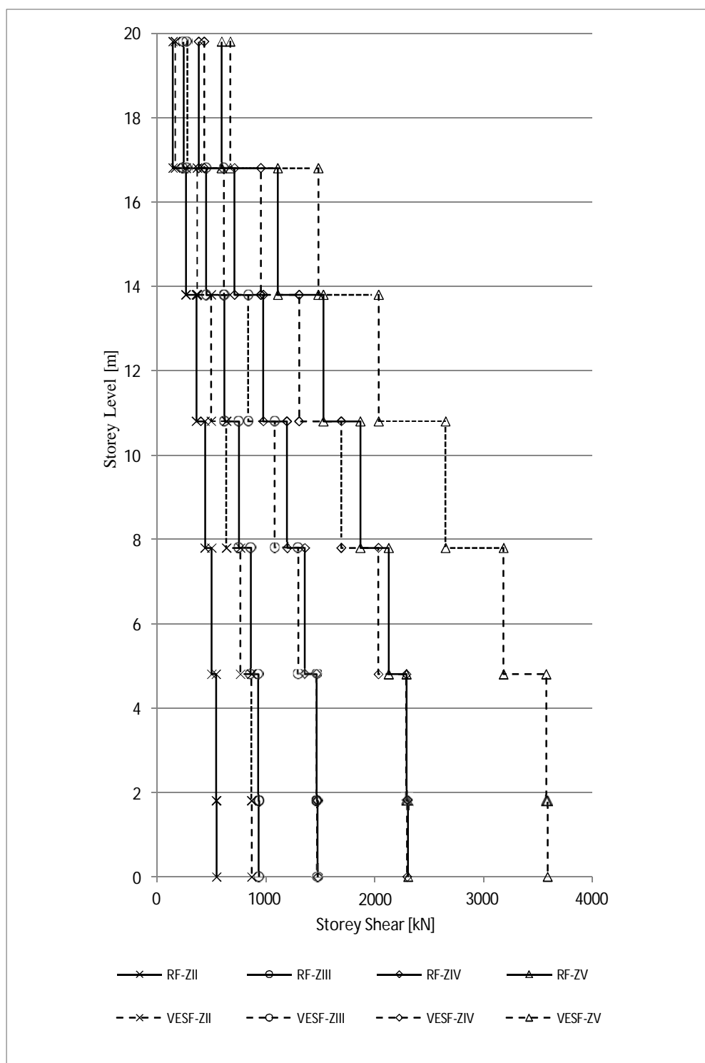
Fig. 4.9 Storey Shear Response of Regular (RF) and Vertical Equal & Single Setback (VESF) Frames under Seismic Loads
