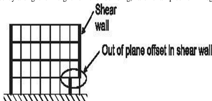
Fig. 1.4 Out of plane Offset Irregularity
