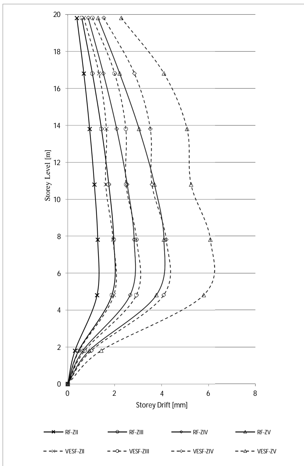
Fig. 4.8 Storey Drift Response of Regular (RF) and Vertical Equal & Single Setback (VESF) Frames under Seismic Loads
