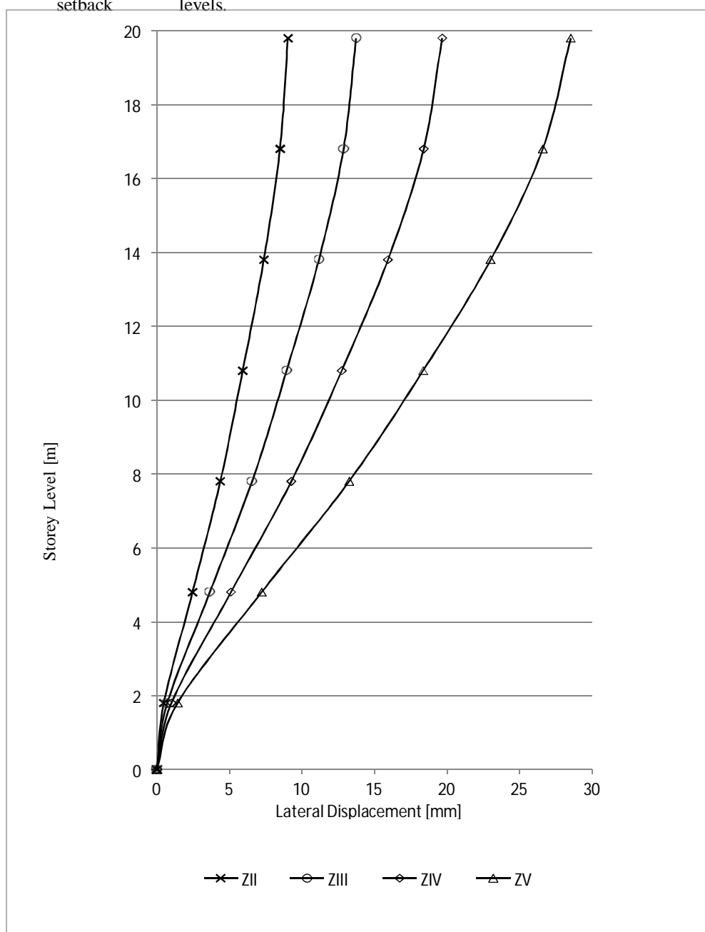
Fig. 4.4 Seismic Response (Lateral Displacement) of Vertical Equal & Single Setback Frame – VESF at all Seismic Zones in India
