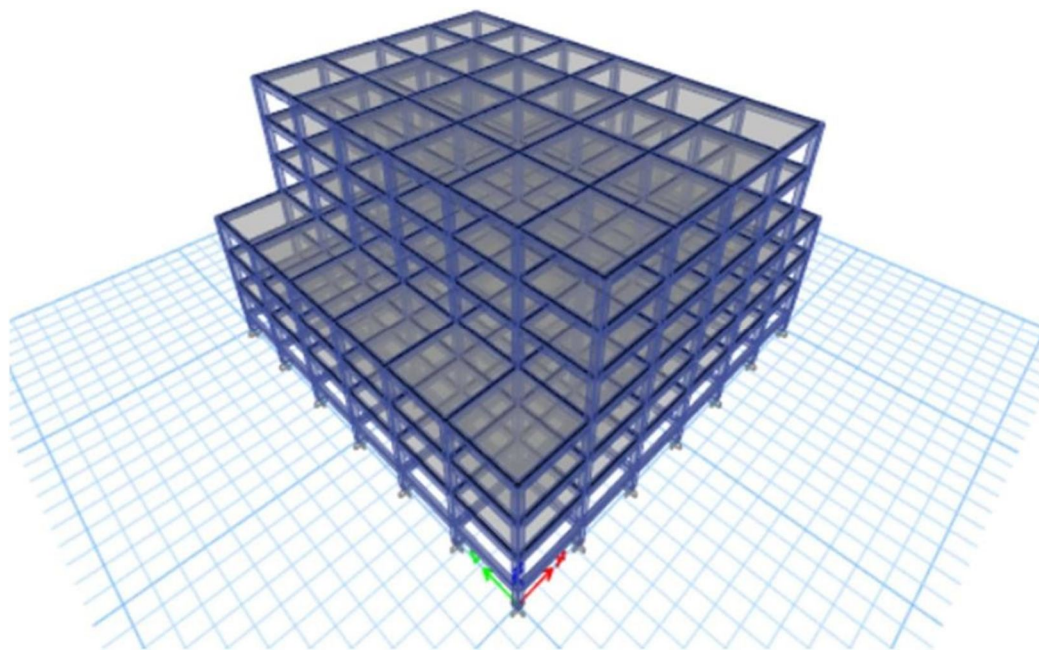
Fig. 3.3 (c) Isometric View of VESF
