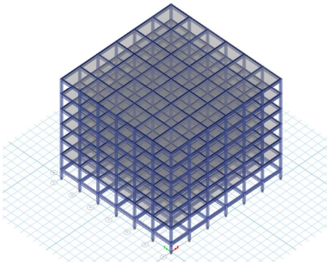
Fig. 3.2 (c) Isometric View of RF
