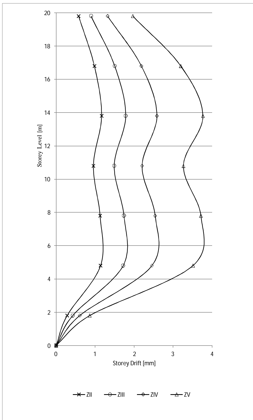
Fig. 4.2 Seismic Response (Storey Drift) of Regular Frame – RF at all Seismic Zones in India
