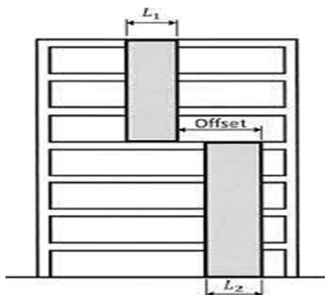
Fig. 1.9 In plane Discontinuity Irregularity
