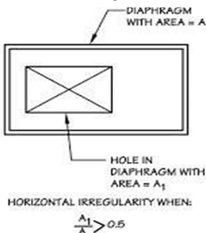
Fig. 1.3 Diaphragm Discontinuity
