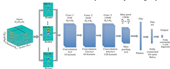
Fig2. CNN Architecture
