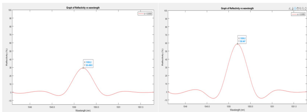
Figure 4 : The reflection spectrum of Fiber Bragg Grating for refractive index change of \Delta n = 0.0003 at grating length of L = 1mm with peak reflectivity, R = 29.45%
