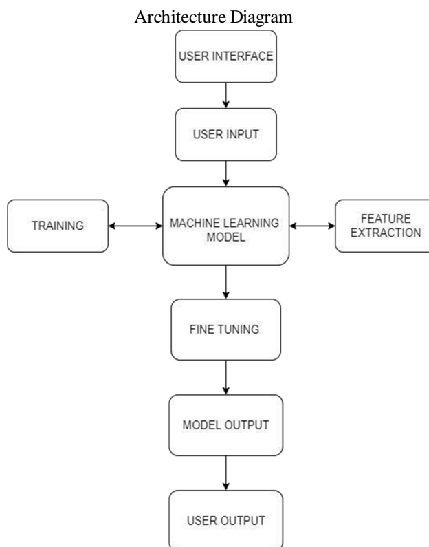
Fig 5- flow diagram
