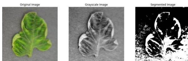
Fig.3.OutputResultOfPlantDiseaseDetection
