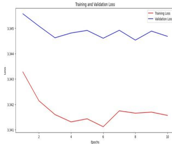
Fig. 1. Train and Valid Loss Graph
