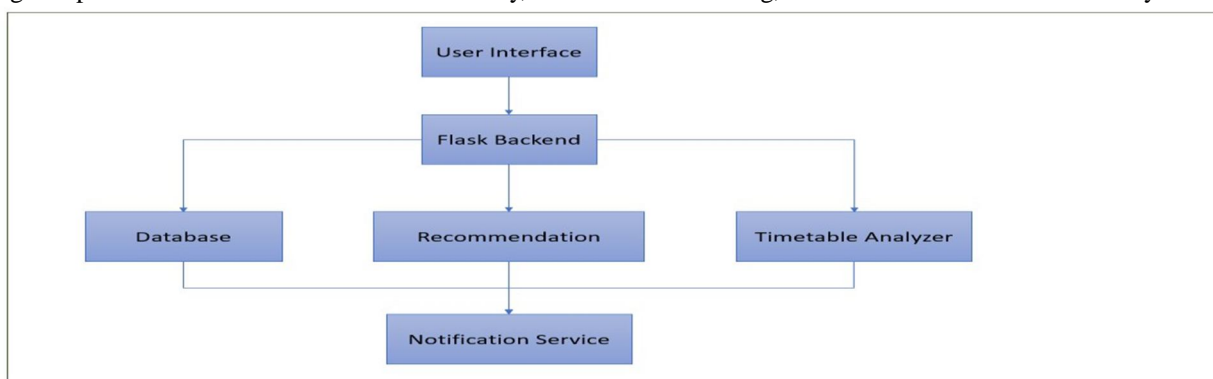
Fig. 1: - System architecture
