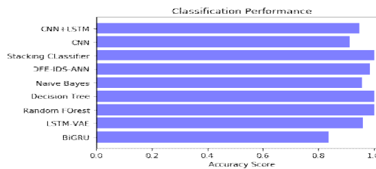
Figure 5 Accuracy graph
