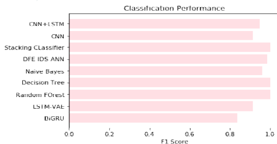
Figure 6 F1Score
