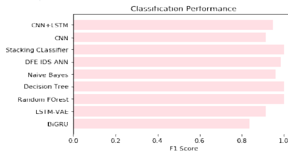
Figure 6 F1Score
