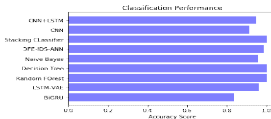
Figure 5 Accuracy graph
