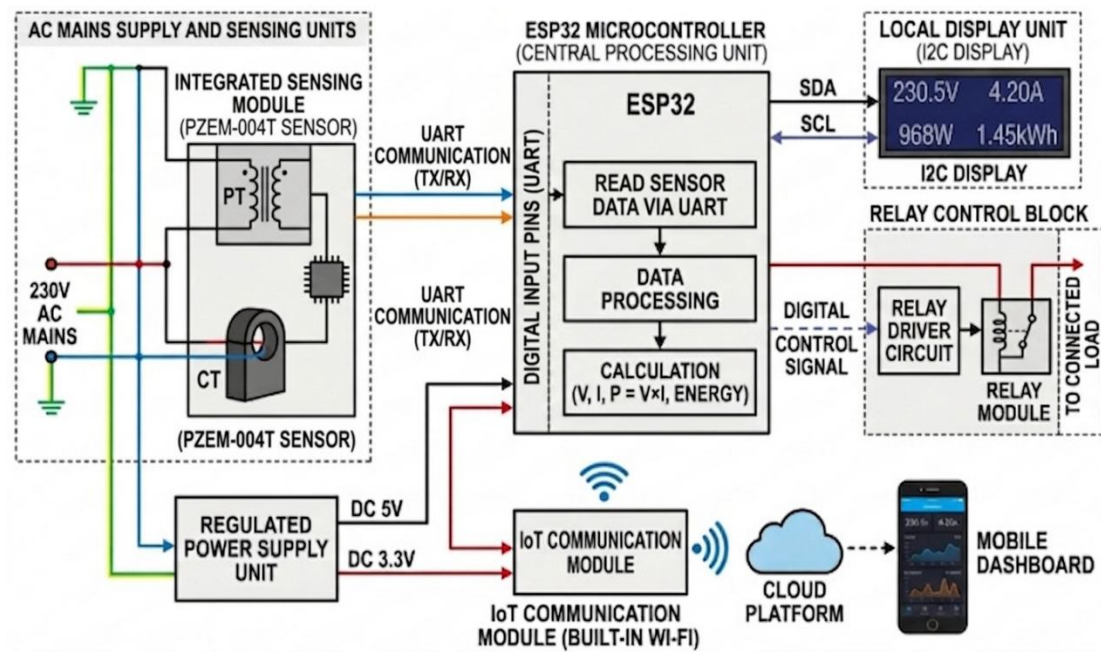
Fig. 1. Block Diagram
