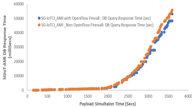
Fig 5: SG-IOT Open-Flow Firewall Full Scale Query Response Behaviour
