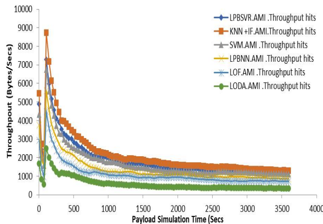
Fig 12: Secure SG-IOT-CI AMI Throughput Validation
