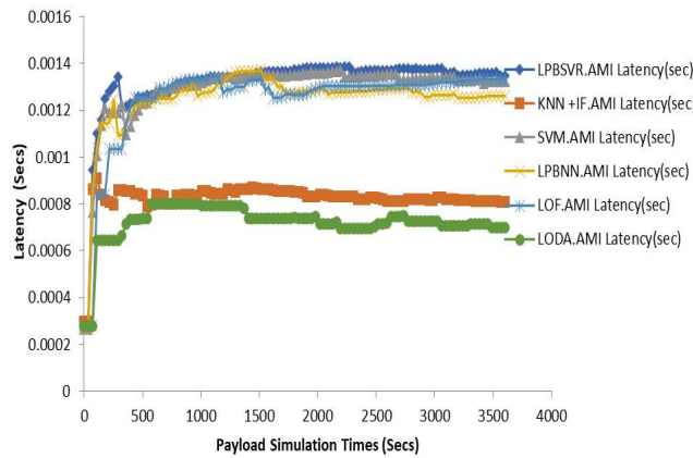
Fig 9 : Secure SG-IOT-CI-AMI Latency (secs)
