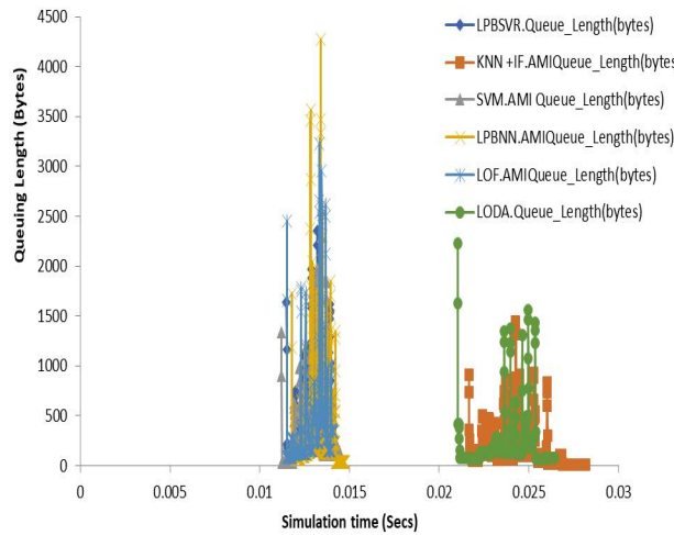
Fig 11: Secure SG-IOT-CI-AMI Queing Workload Validation
