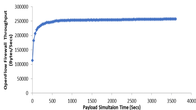
Fig 7: SG-IOTCI AMI Throughput with OpenFlow Firewall
