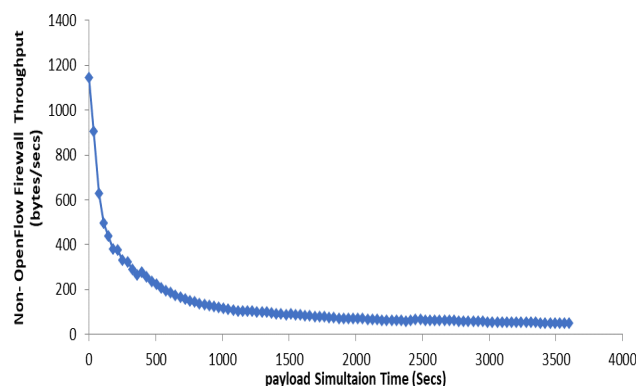
Fig 8 : SG-IOTCI AMI Throughput with Non-Openflow Firewall
