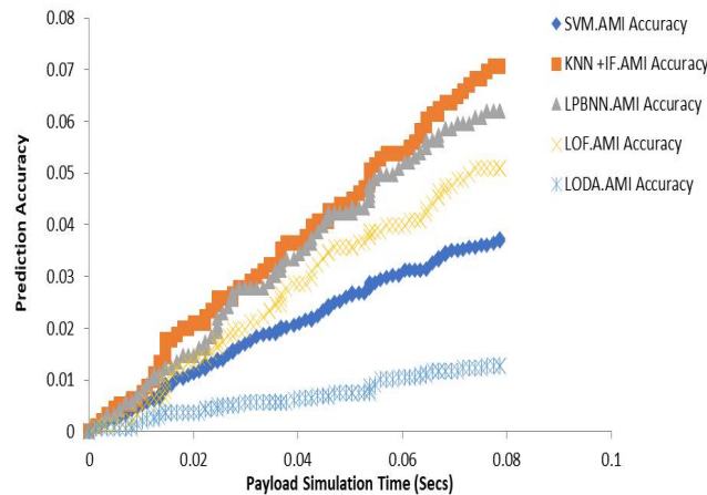
Fig 13: Secure SG-IOT-CI-AMI Accuracy Validation
