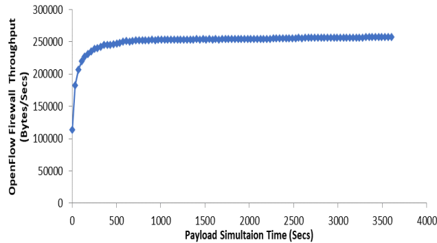
Fig 7: SG-IOTCI AMI Throughput with OpenFlow Firewall
