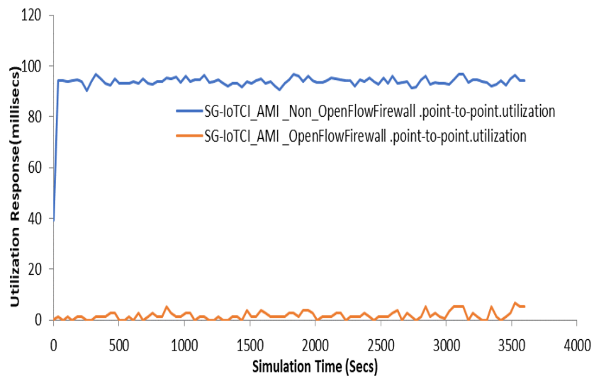
Fig 6: SG-IOT Open Flow Firewall Resource Consumption During Tampering
