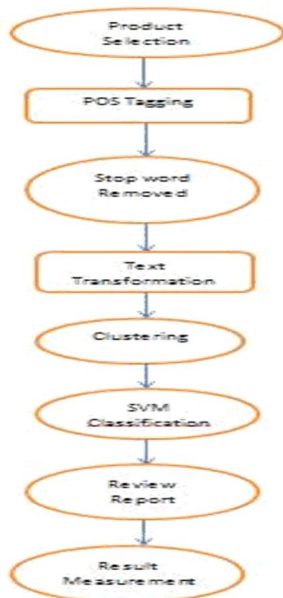
Figure 3.1: Flow of proposed methodology has been consisting various phases.
