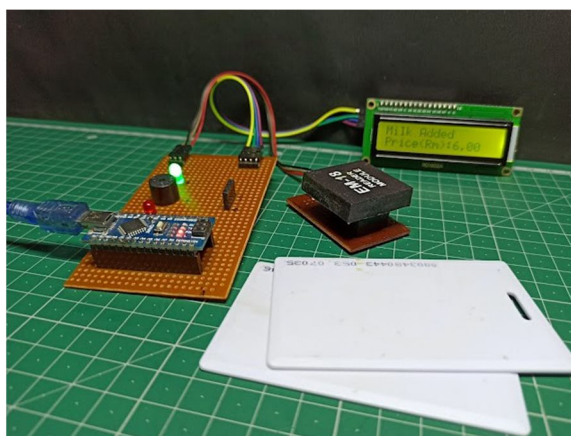
Fig 3: Working Smart Card Circuit.
