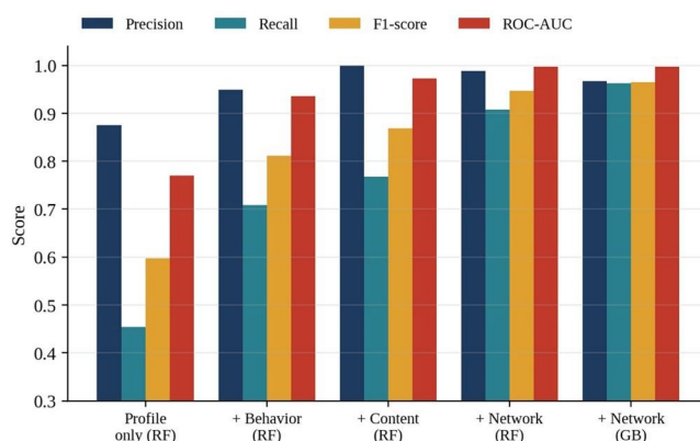
Fig. 2. Effect of adding signal families on detection quality (synthetic data).
