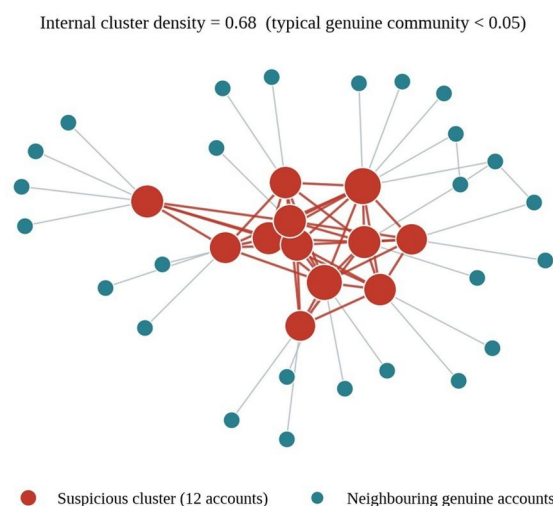
Fig. 6. A suspicious account cluster detected by community analysis (synthetic data). Node size reflects PageRank within the subgraph.
