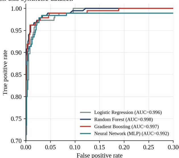
Fig. 3. ROC curves of the four model families (synthetic data; axes zoomed).
