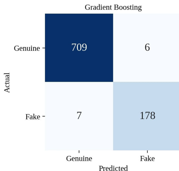
Fig. 4. Confusion matrix of the best-scoring model (Gradient Boosting).
