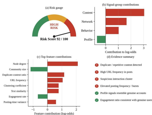
Fig. 5. Example investigation report with risk gauge, signal-group contributions, feature contributions and evidence (synthetic data; illustrative).
