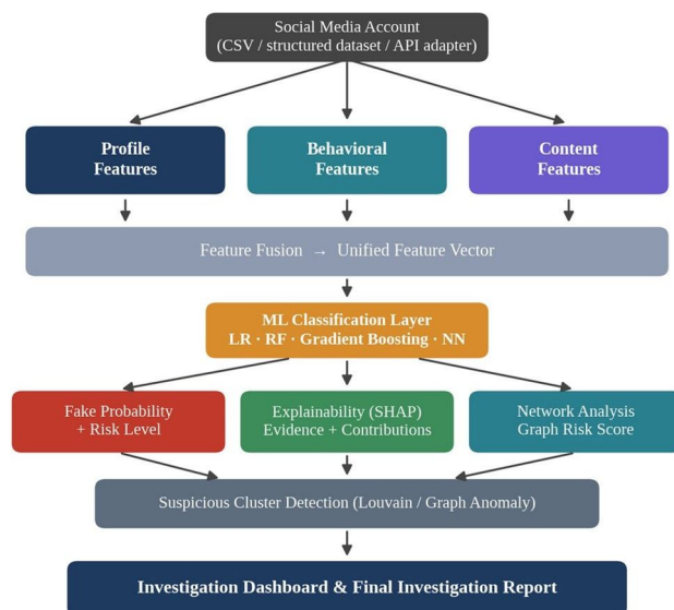
Fig. 1. Architecture of the proposed SocialGuard framework.
