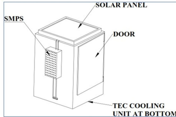
Fig 4. Design of solar refrigerator
