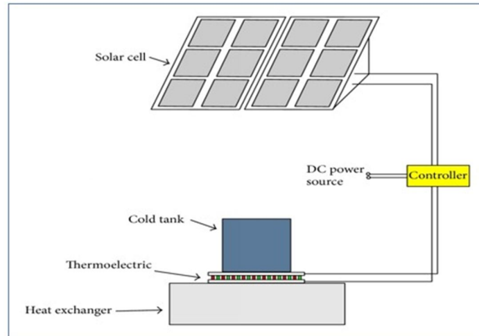
Fig.3 Assembly of System
