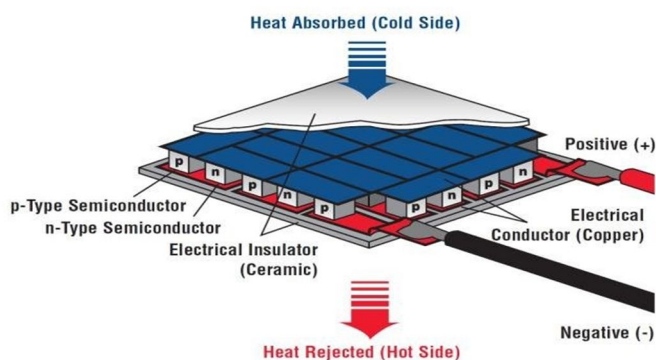
Fig.1 Structure of Peltier module
