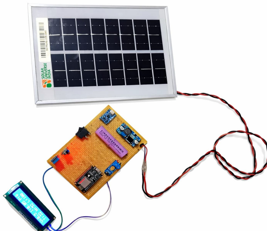
Fig.1 Solar panel with mounted sensors during outdoor field testing
