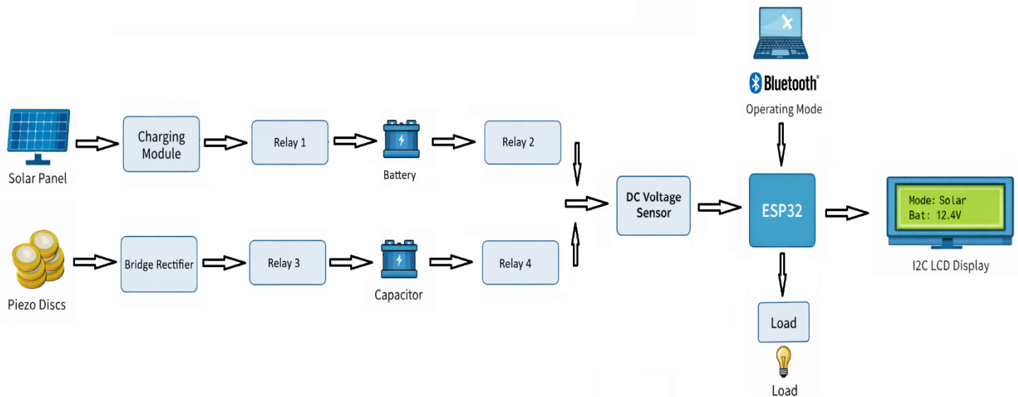
Fig.1.BLOCKDIAGRAM
