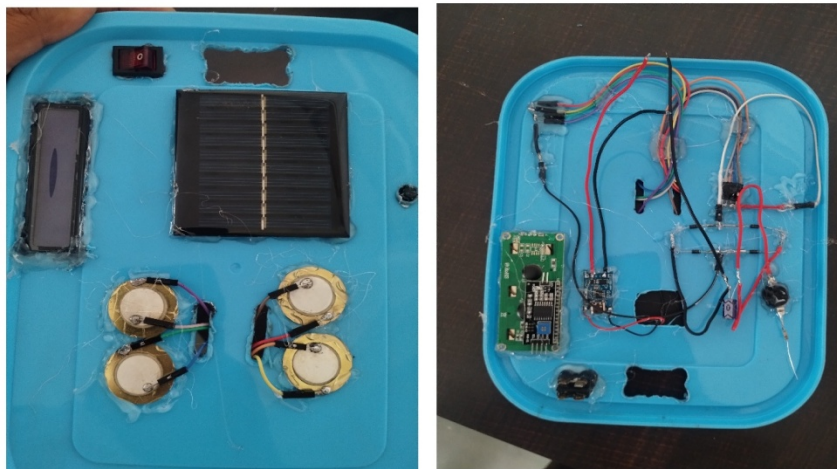
Fig.2.KIT PHOTO
