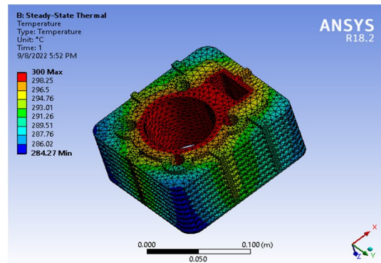
Fig 9 : Fins Al 6061 materials temperature at 300°C steady
