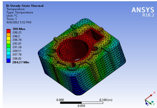
Fig 9 : Fins Al 6061 materials temperature at 300 0 C steady
