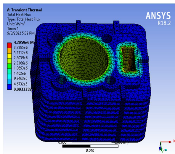
Fig.6 Fins Al 6061 materials total heat flux at 300 0 C transient
