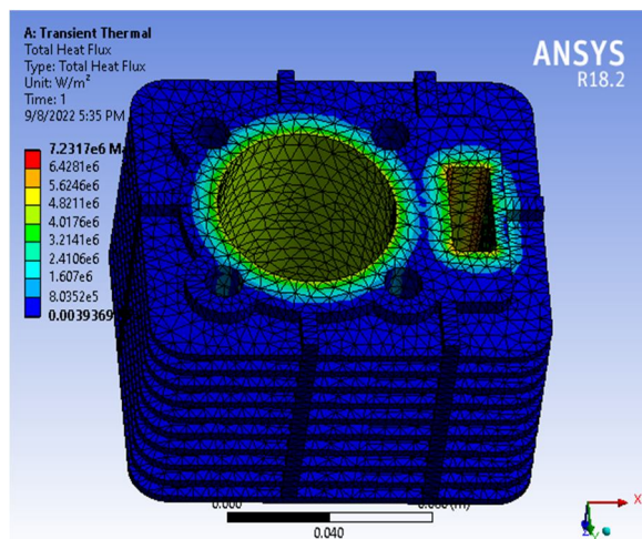
Fig.12: Fins Al 6061 materials total heat flux at 500 0 C transient
