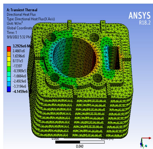
Fig.4 Fins Al 6061 materials directional heat flux transient at 300 °C
