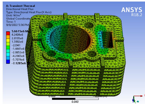
Fig. 10 Fins Al 6061 materials directional heat flux at 500 0 C transient
